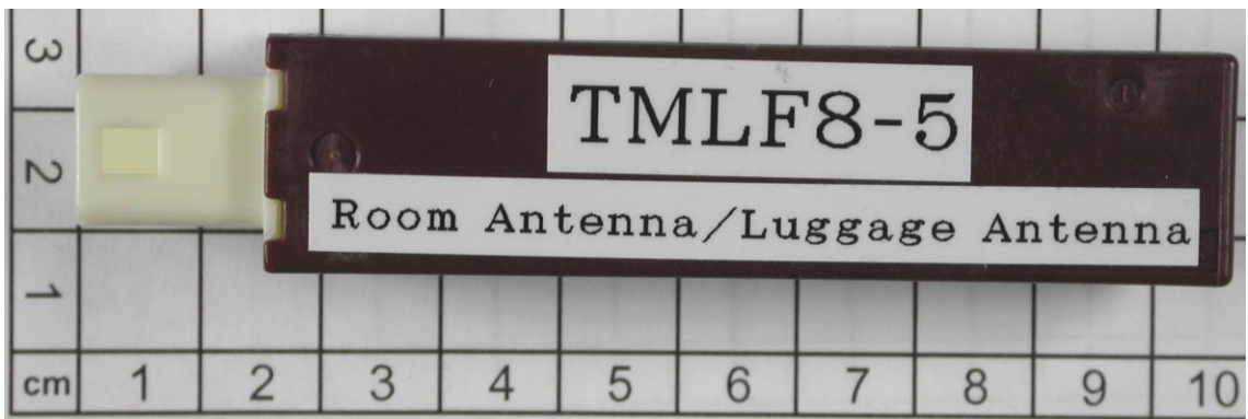
Room Antenna:
