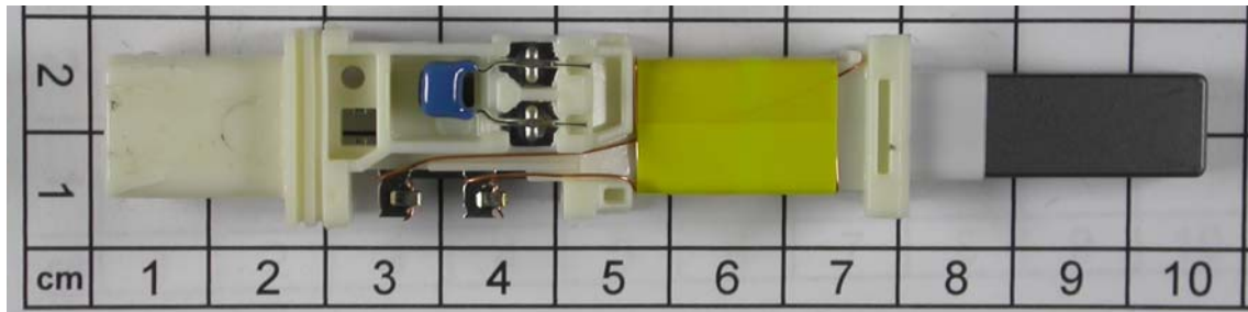
Room antenna 8RA
