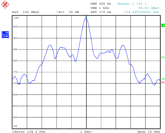
Trunk antenna
