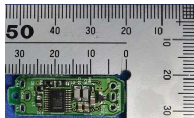
Rear View
