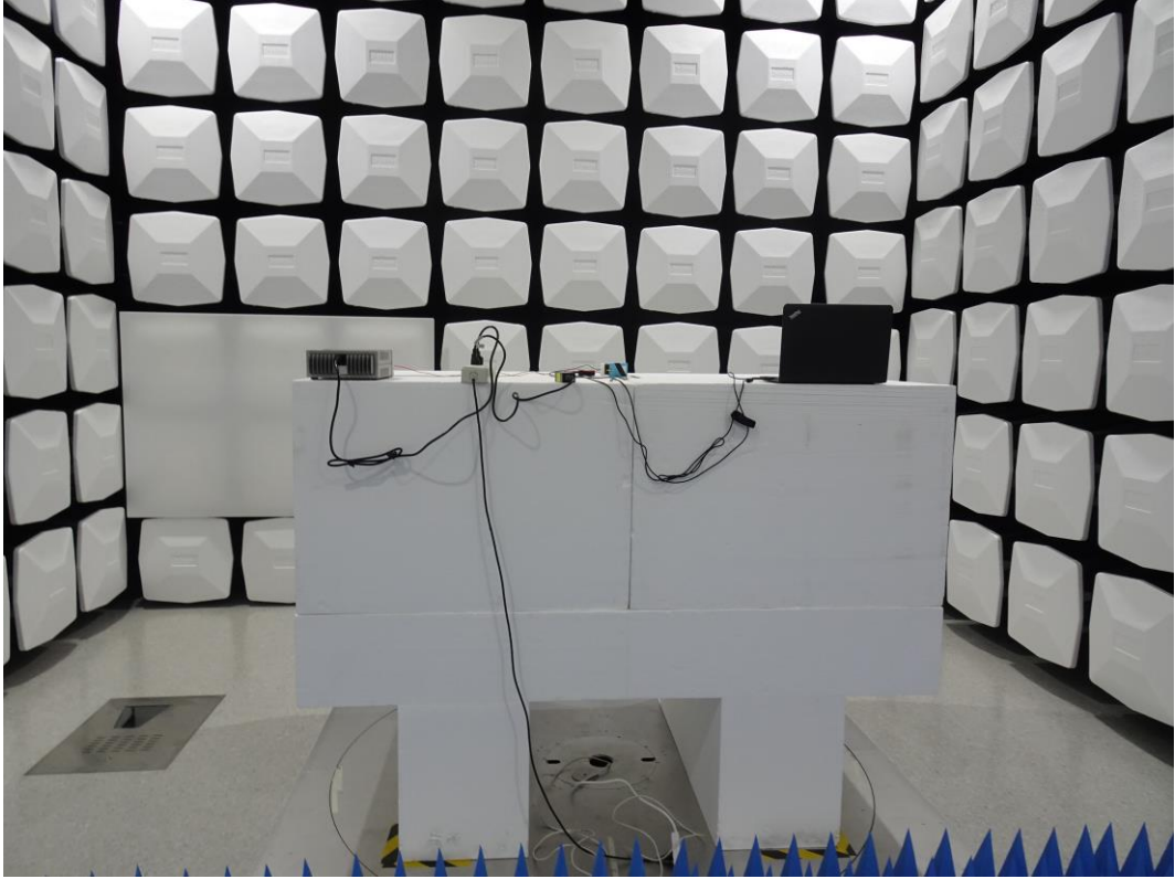
Back View of Radiated Emission Test (Horn)
