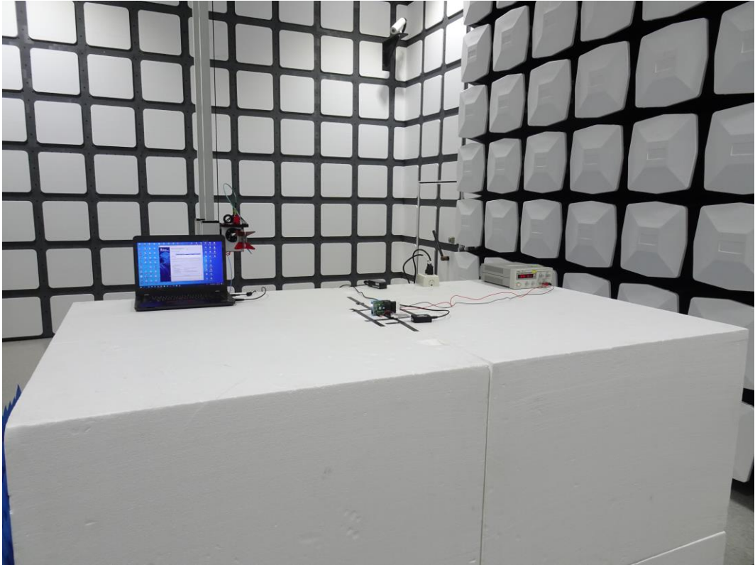
Front View of Radiated Emission Test (Horn)
