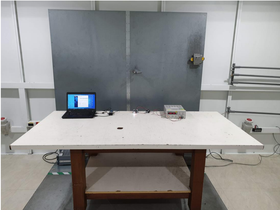
Front View of Conducted Emission Test
