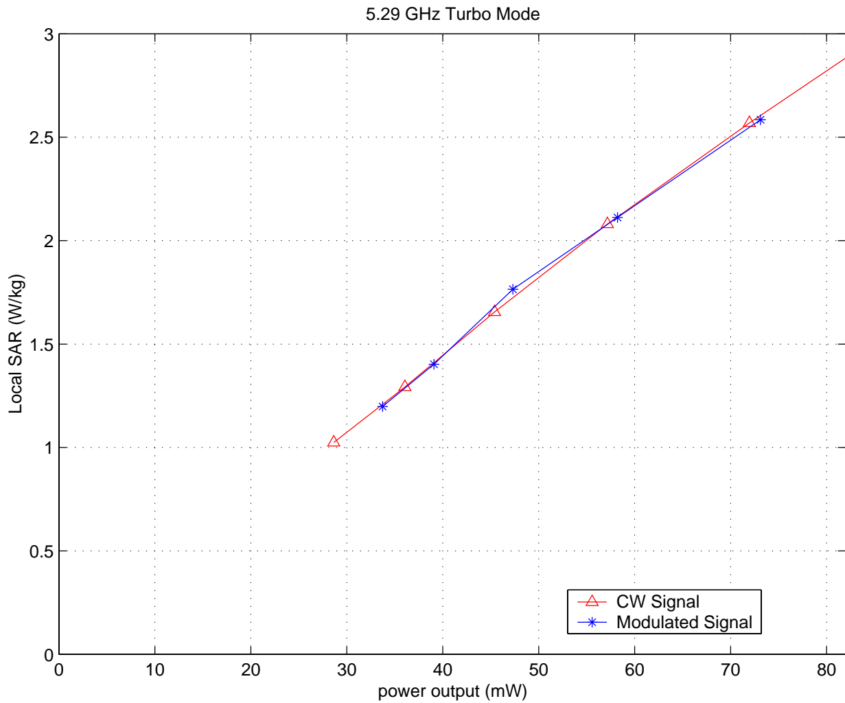
Fig. A.1. Comparison of the SAR for CW or OFDM modulated signals for the turbo mode at 5.29 GHz.
