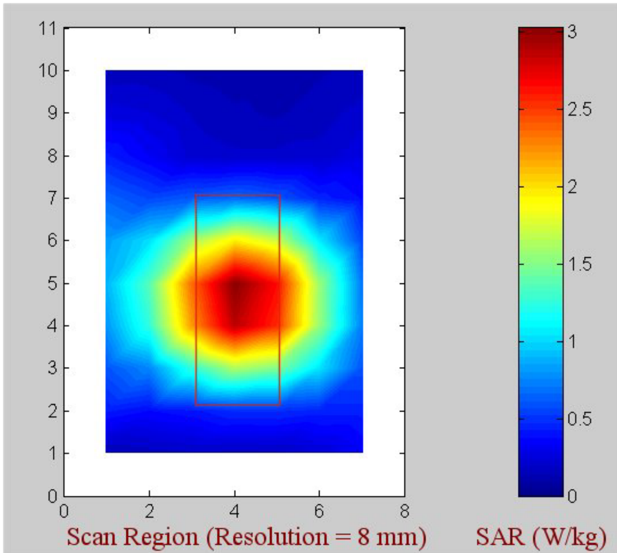
Fig. B.1. Coarse scans of the measured SAR distribution for the WR187 rectangular waveguide irradiation system for system verification at 5.25 GHz. Also shown is the outline of the rectangular waveguide overlaid on the SAR contours. Radiated power = 100 mW.
