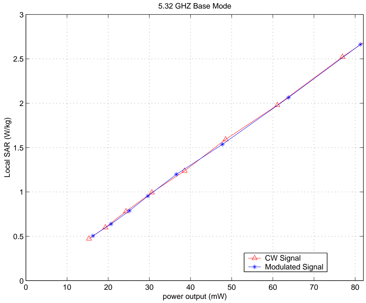
Fig. A.2. Comparison of the SAR for CW or OFDM modulated signals for the base mode at 5.32 GHz.
