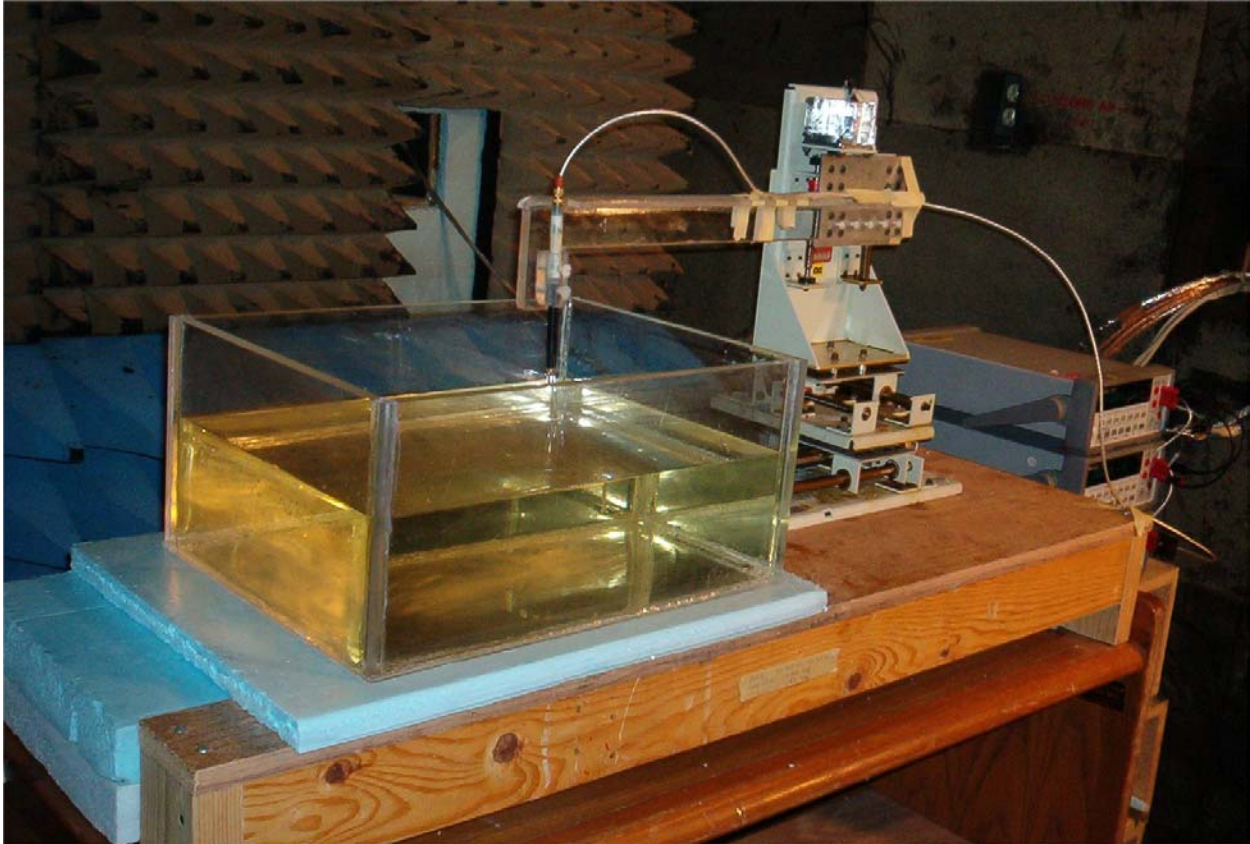
Fig. 4. Photograph of the three-dimensional stepper-motor-controlled SAR measurement system using a planar phantom (see Figs. 2 and 3 for a detailed examination of the placement of the IBM Model 2659 Notebook Computer with Senao Wireless Cardbus Adapter Model SL-5354CB relative to this phantom).
