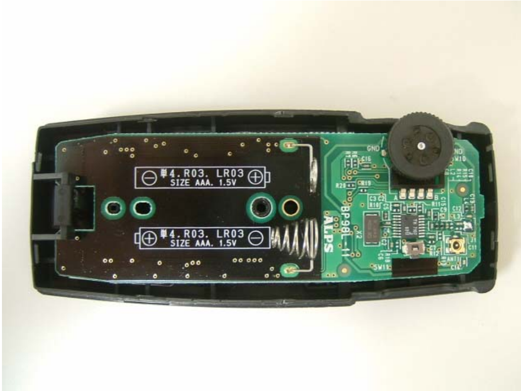
Open View (Top)
