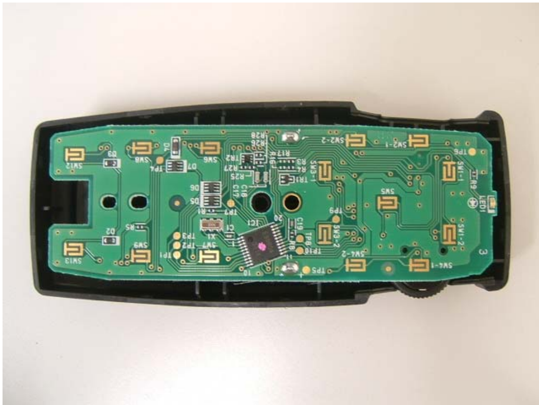
Open View (Bottom)
