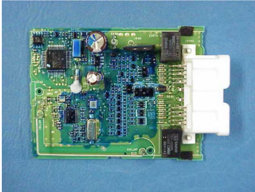
Circuit board <Front>
