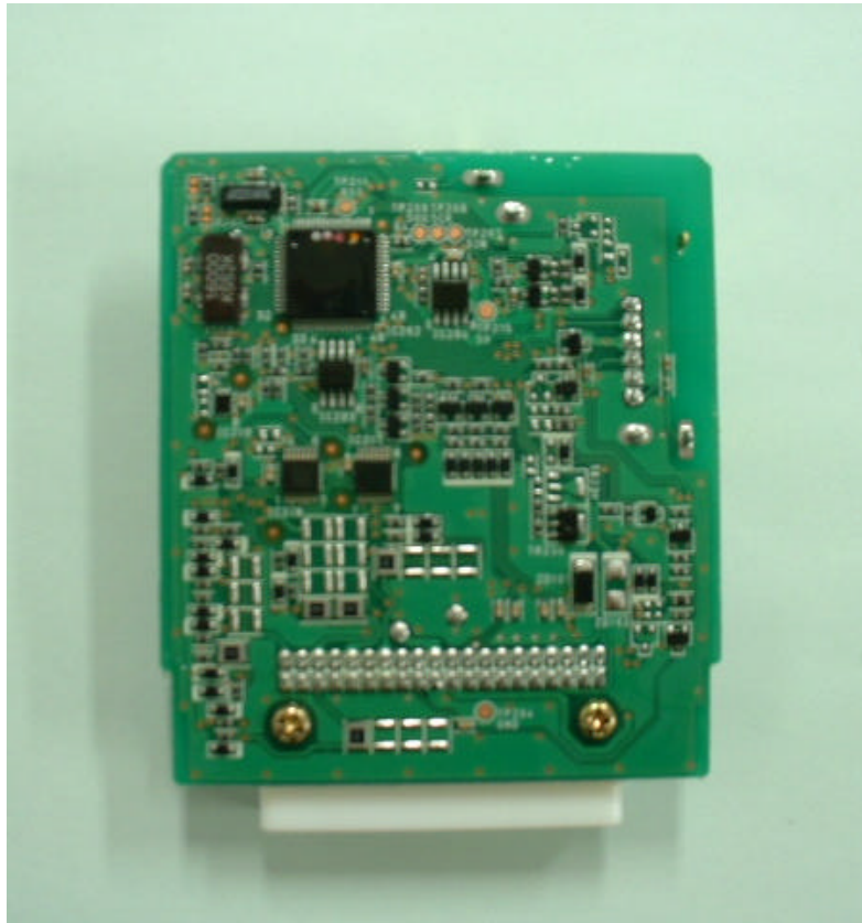
Circuit board<rear view>
