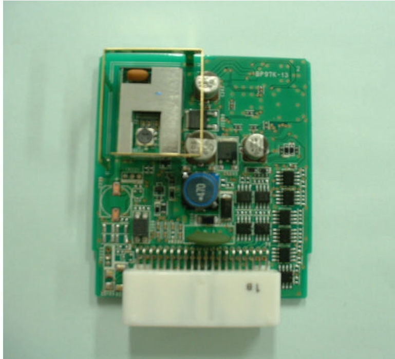
Circuit board<front>
