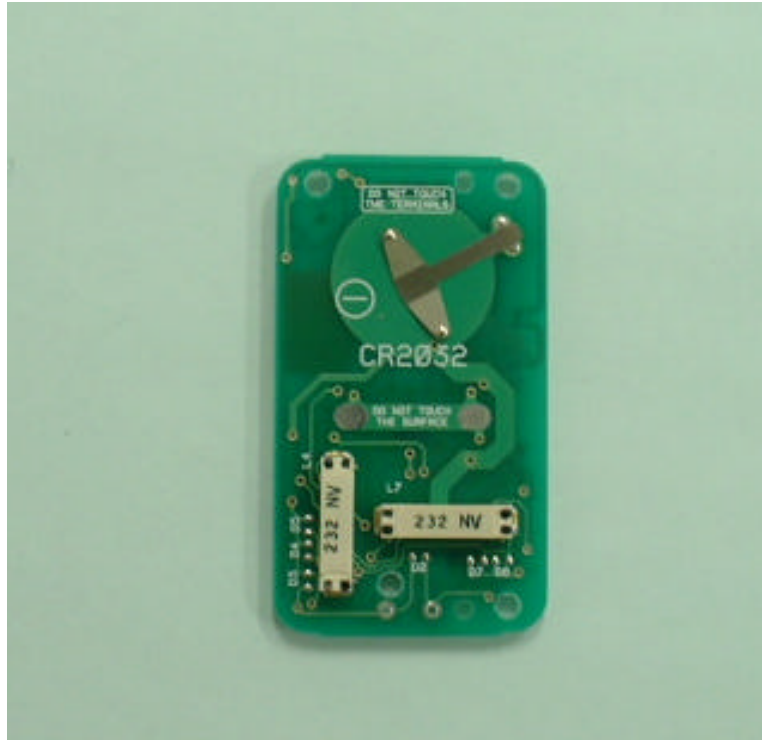
Circuit board<rear >
