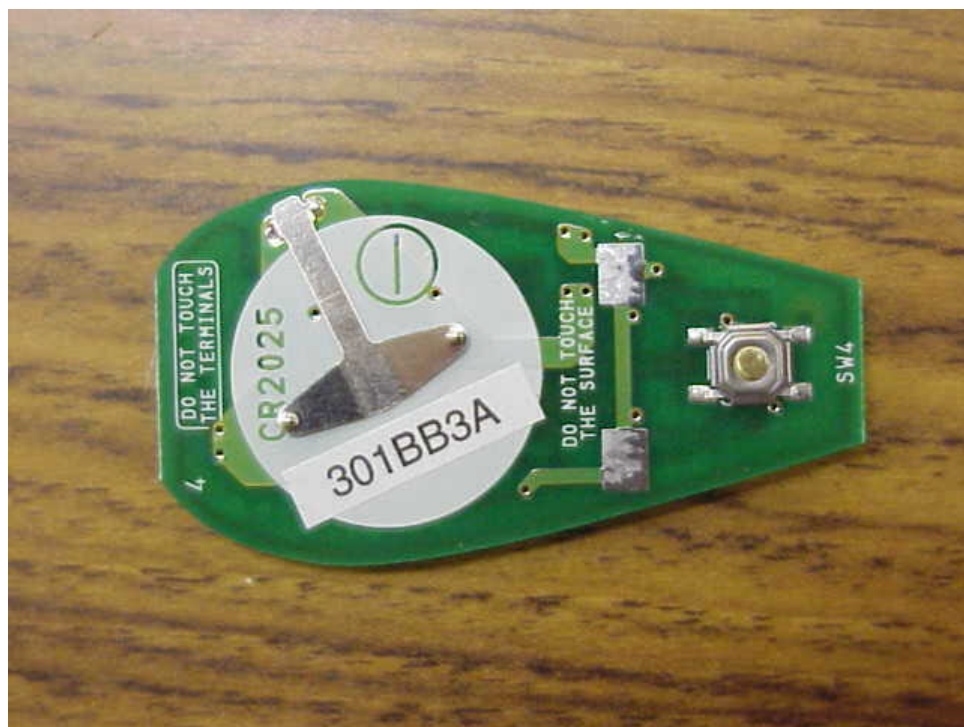
PCB Side B
