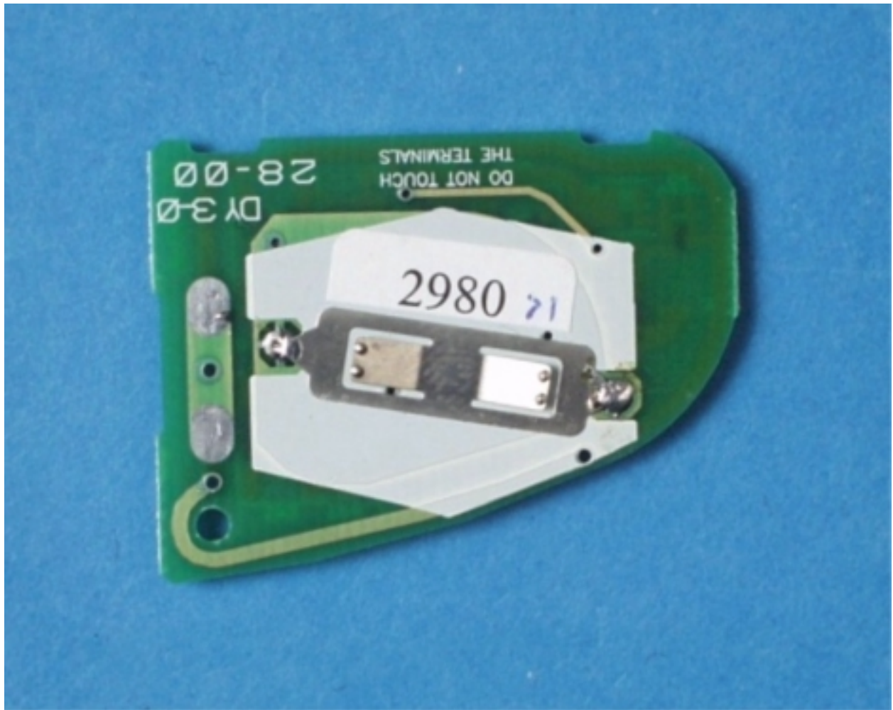
Circuit Board, Circuit Side
