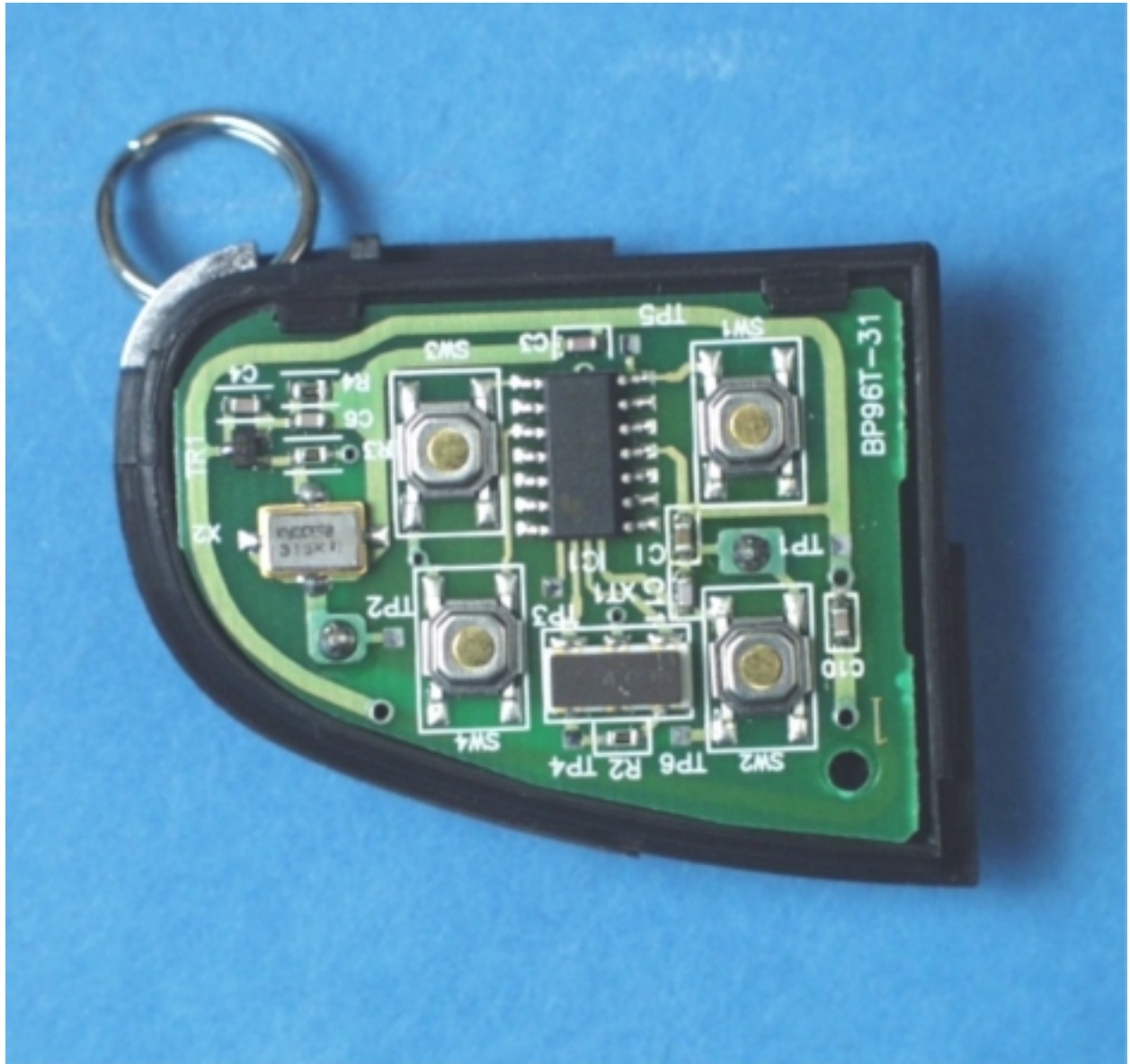
Circuit Board, Component Side
