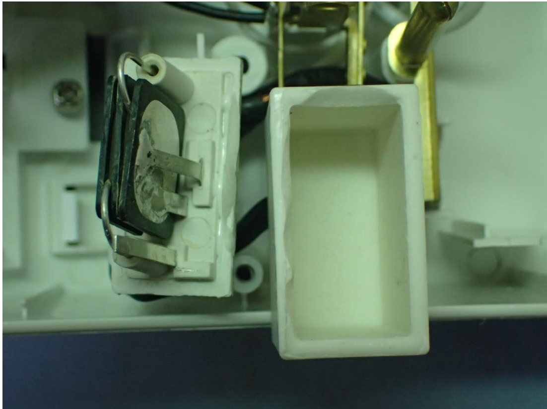
Figure 23 For Surge Protector 1080J Model, Internal View
