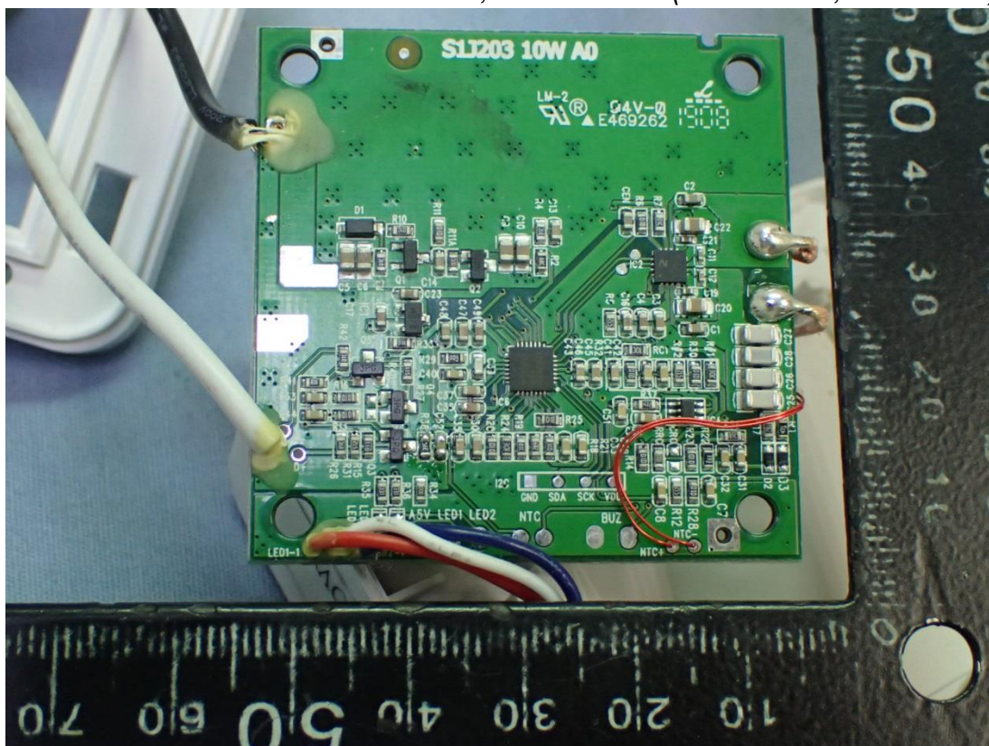
Figure 34 For all Models, Internal View (WPC Board, Front View)
