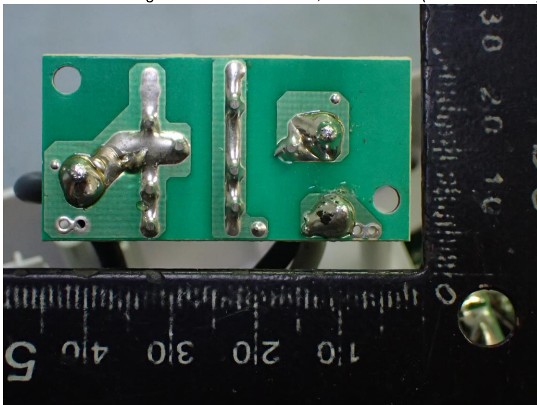
Figure 21 For Surge Protector 860J Model, Internal View (PCB Back View)
