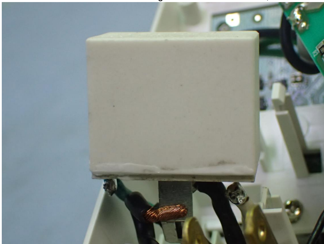
Figure 22 For Surge Protector 1080J Model, Internal View
