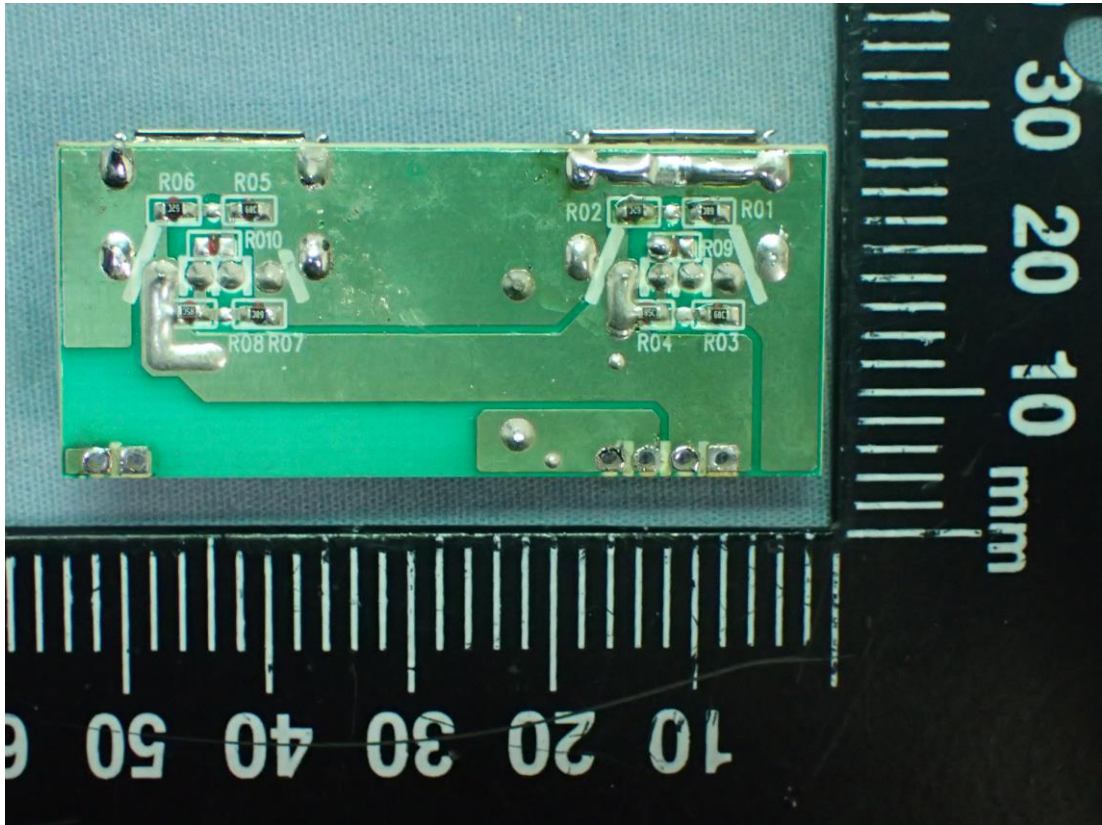
Figure 17 For all Models, Internal View (USB Board, Back View)
