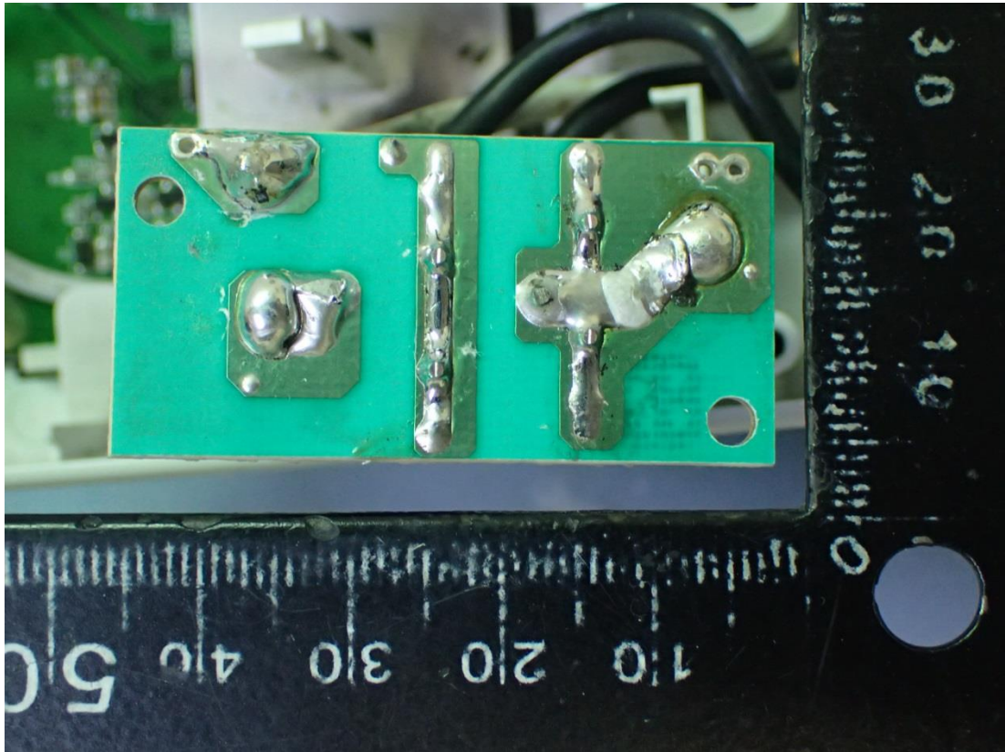
Figure 19 For Surge Protector 560J Model, Internal View (PCB Back View)
