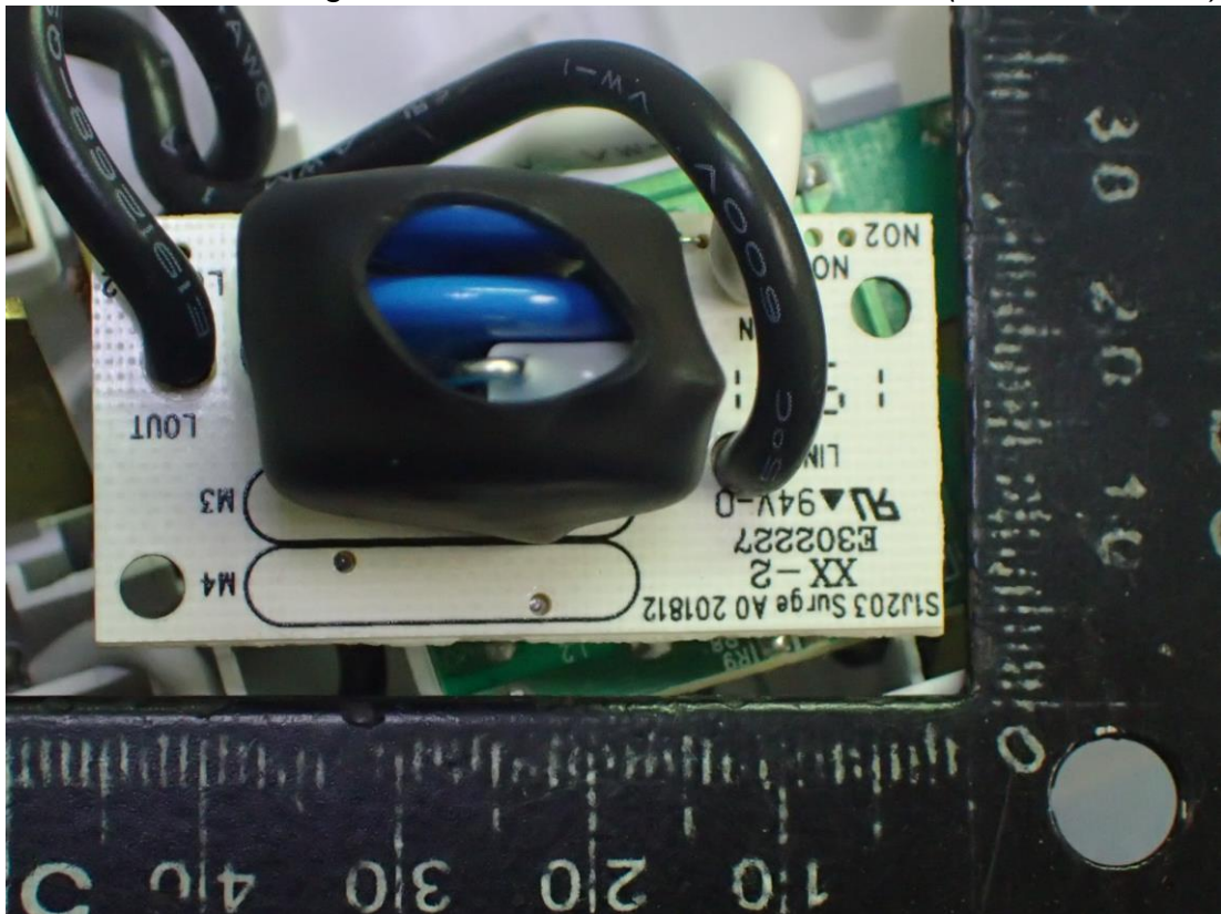
Figure 20 For Surge Protector 860J Model, Internal View (PCB Front View)
