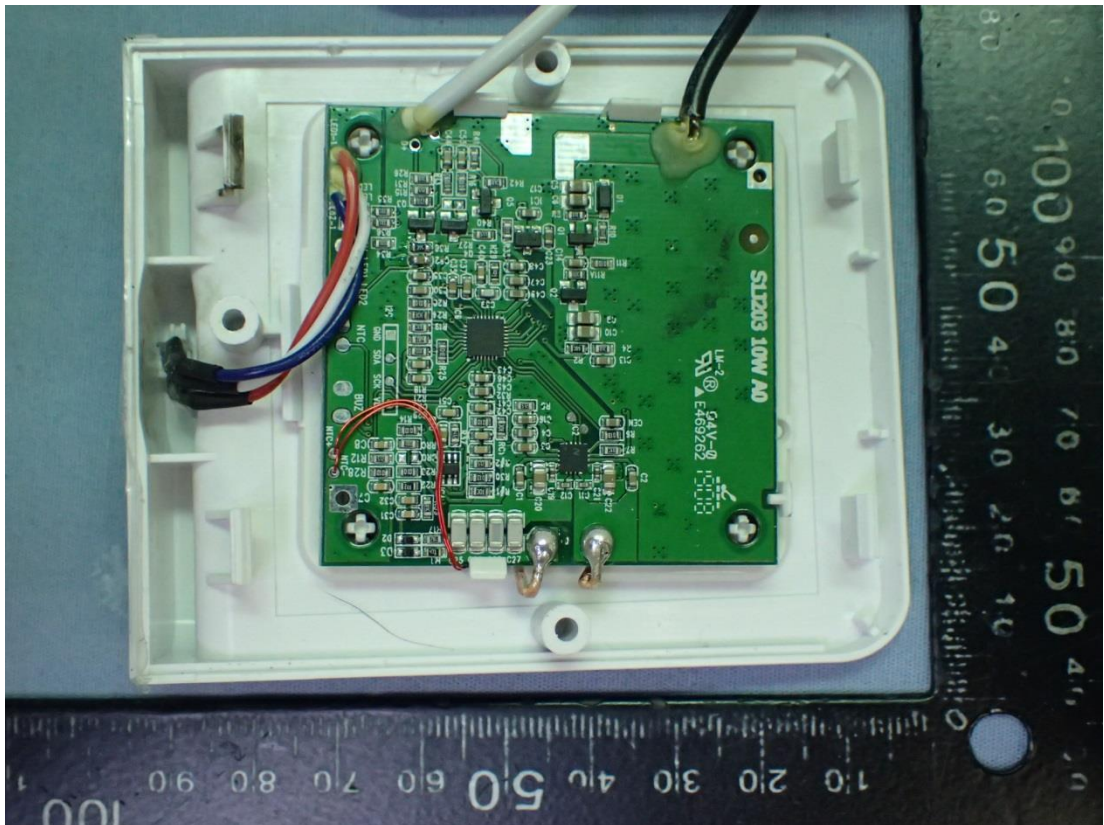
Figure 30 For all Models, Internal View
