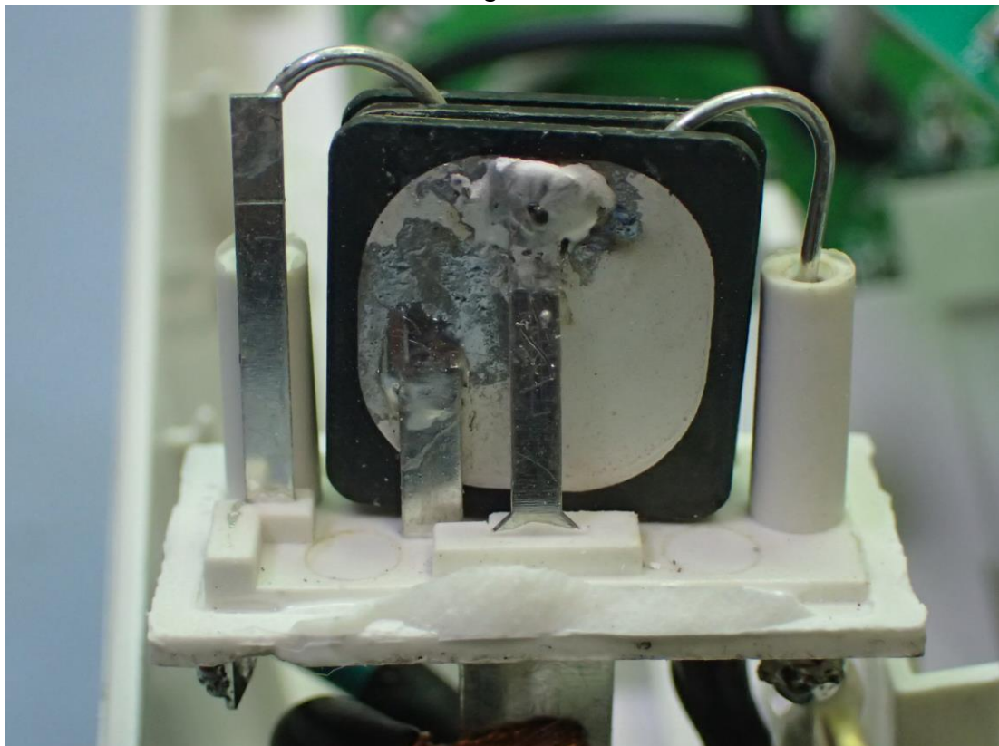
Figure 24 For Surge Protector 1080J Model, Internal View
