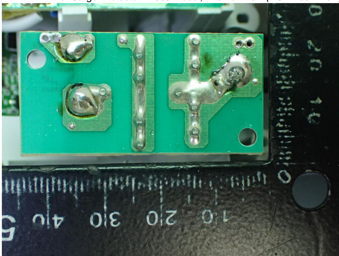
Figure 27 For Surge Protector 1200J Model, Internal View (PCB Back View)
