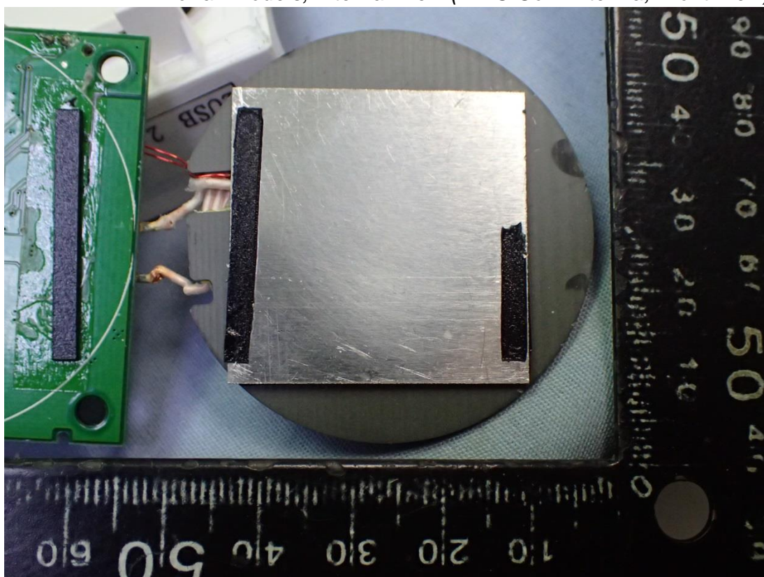
Figure 33 For all Models, Internal View (WPC Coil Antenna, Front View)
