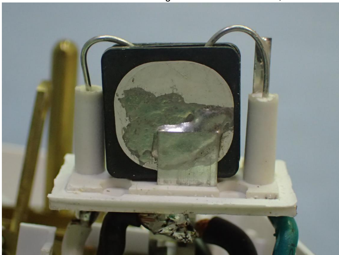
Figure 25 For Surge Protector 1080J Model, Internal View
