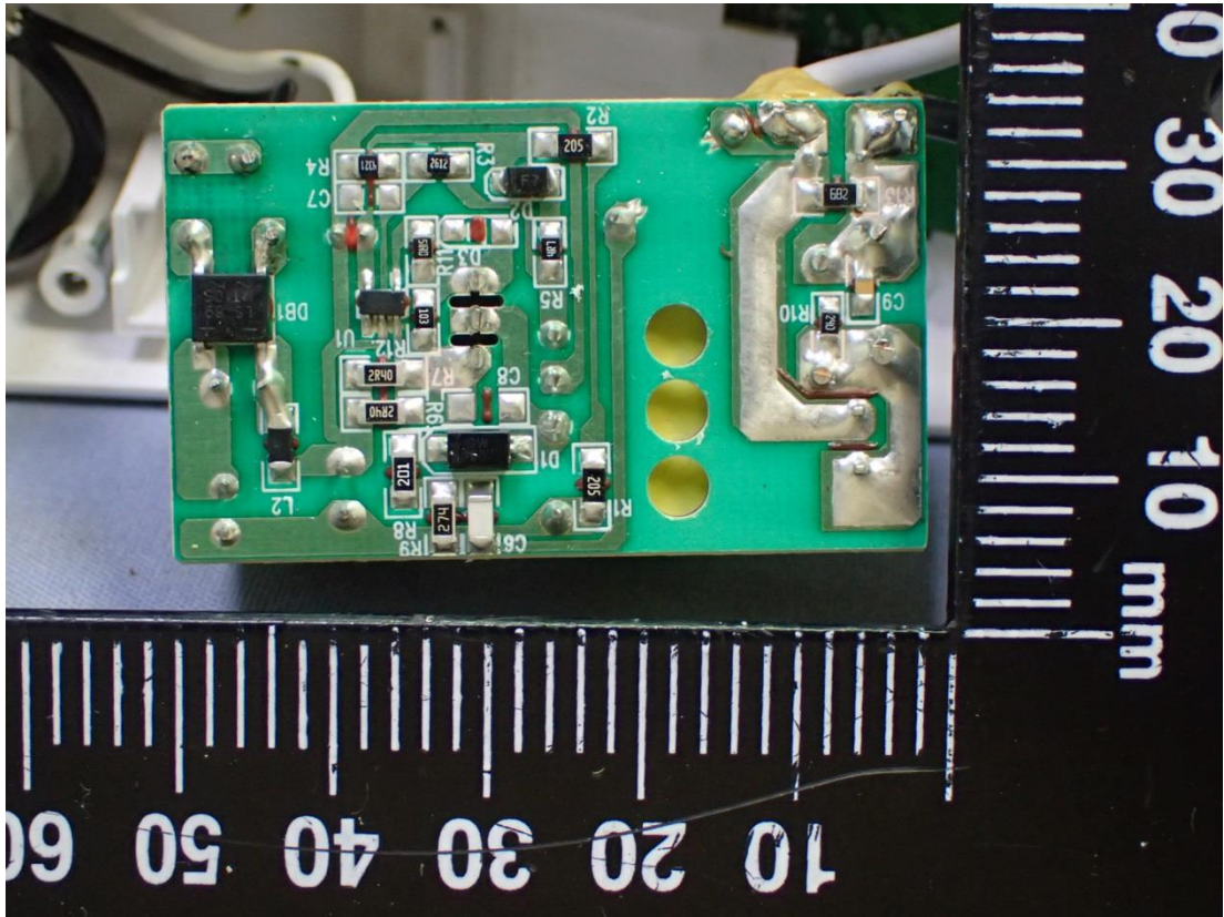
Figure 29 For all Models, Internal View (PCB Front View)
