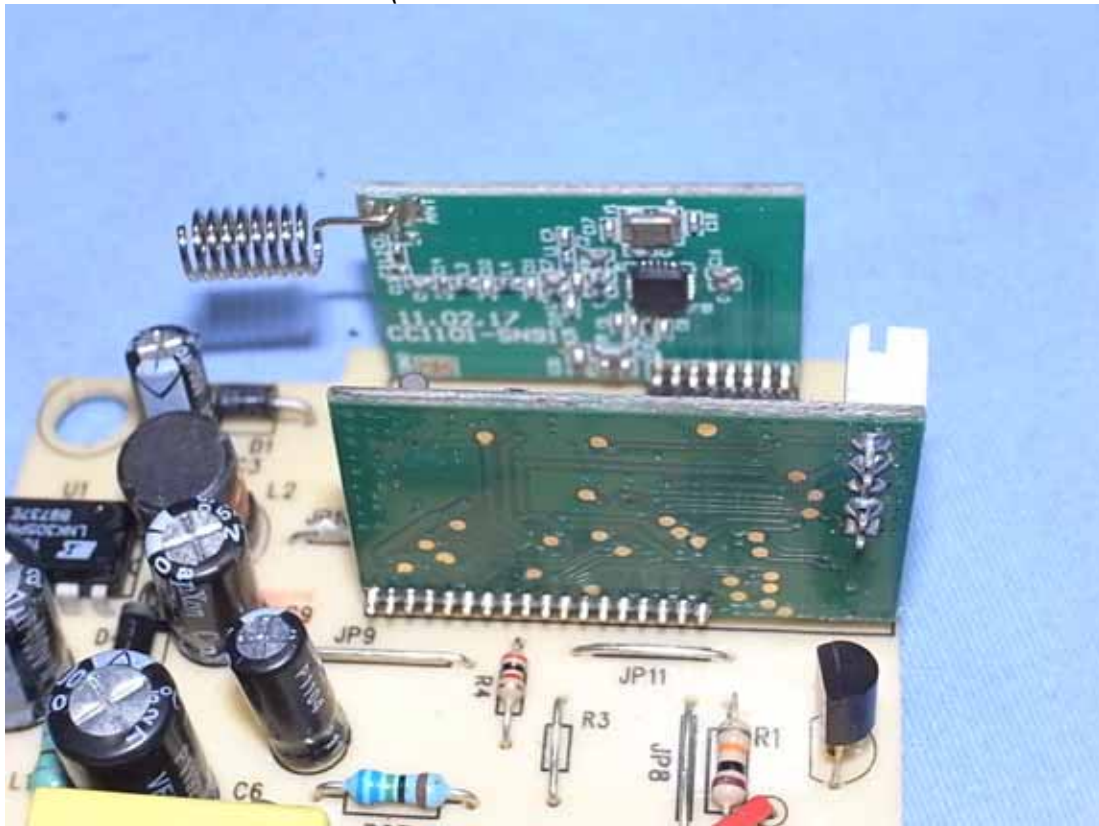
Photo 9 Internal View (Control Board/Back View & RF Module Board/Front View)
