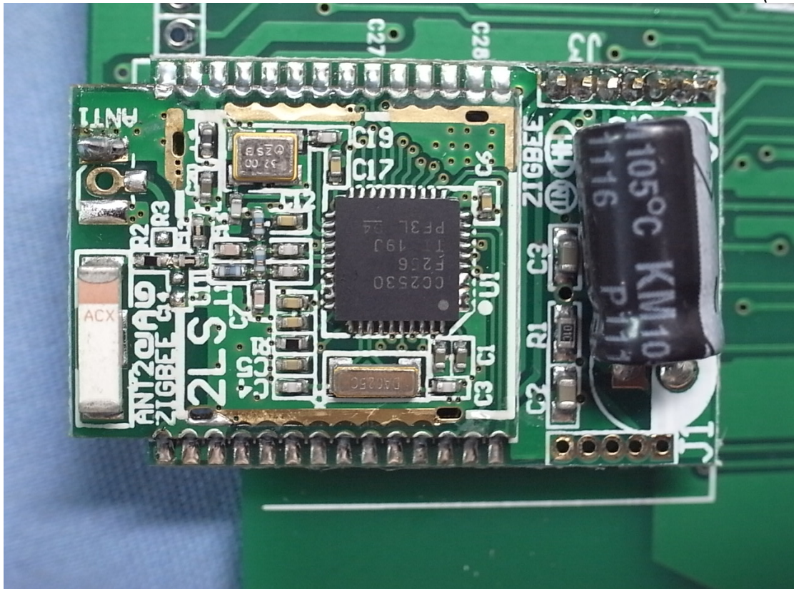
Photo 9 Internal View (RF Board)
