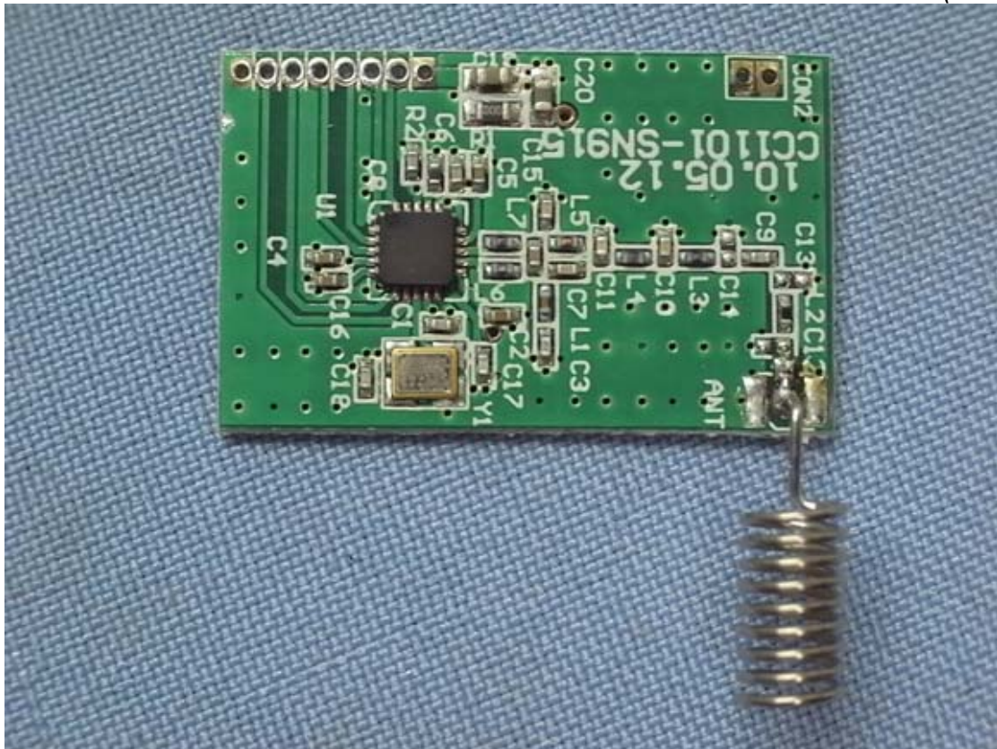
Photo 12 PCB View (Front View)
