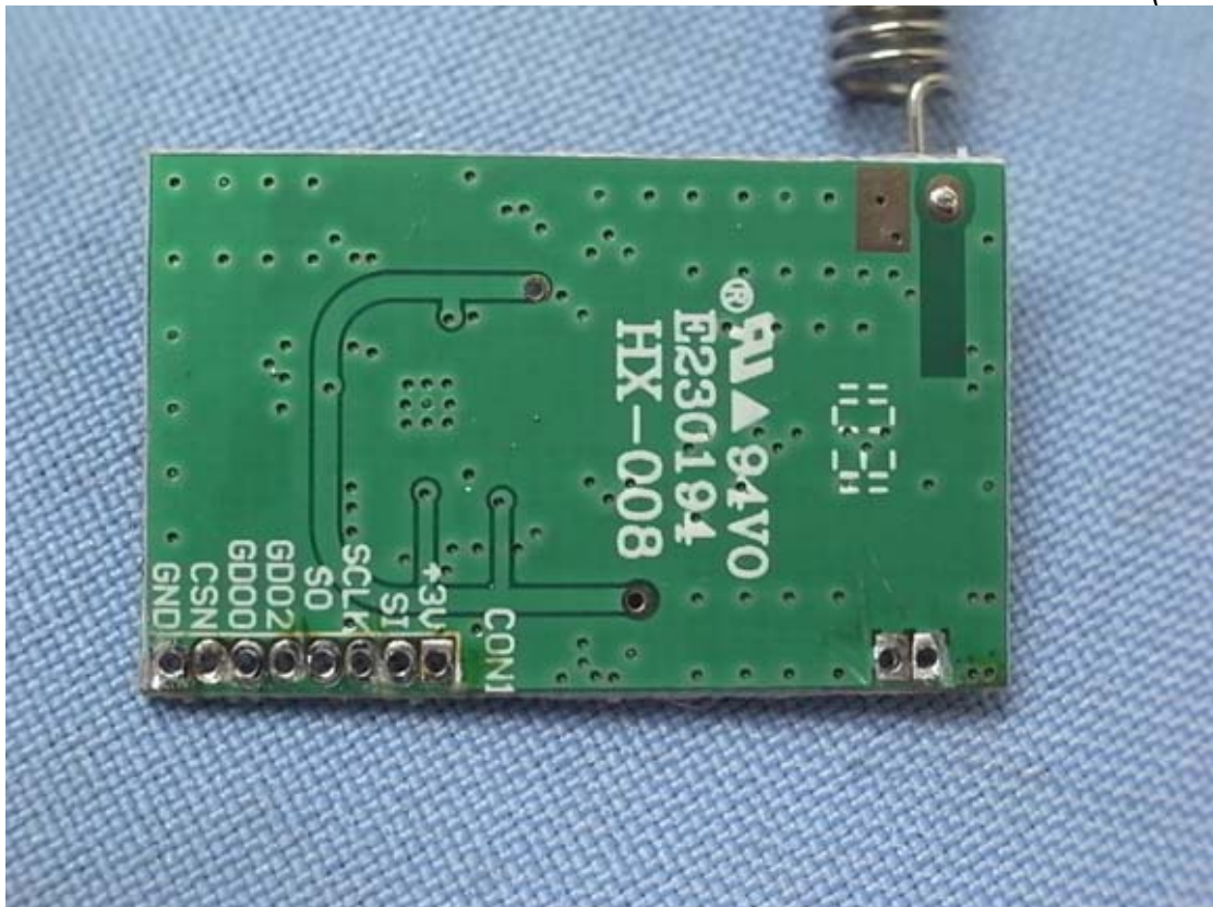
Photo 13 PCB View (Back View)
