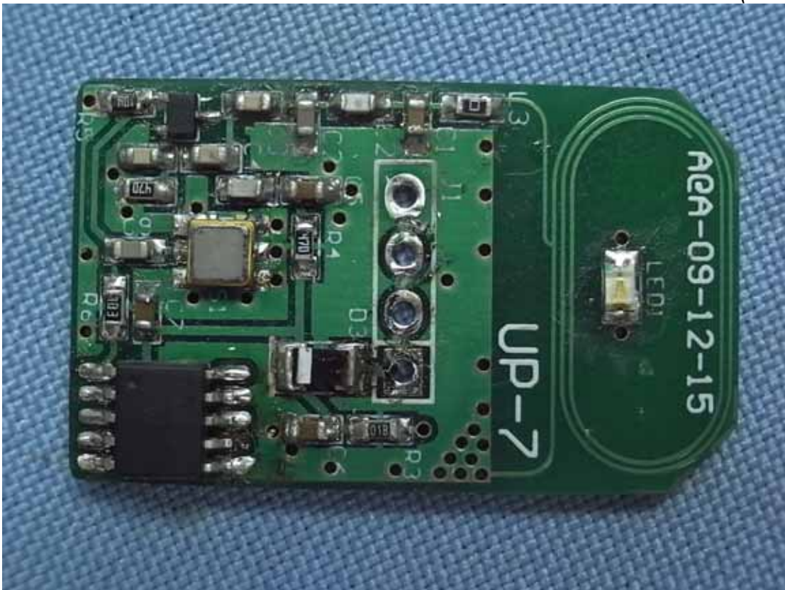
Photo 6 PCB View (Front Side)
