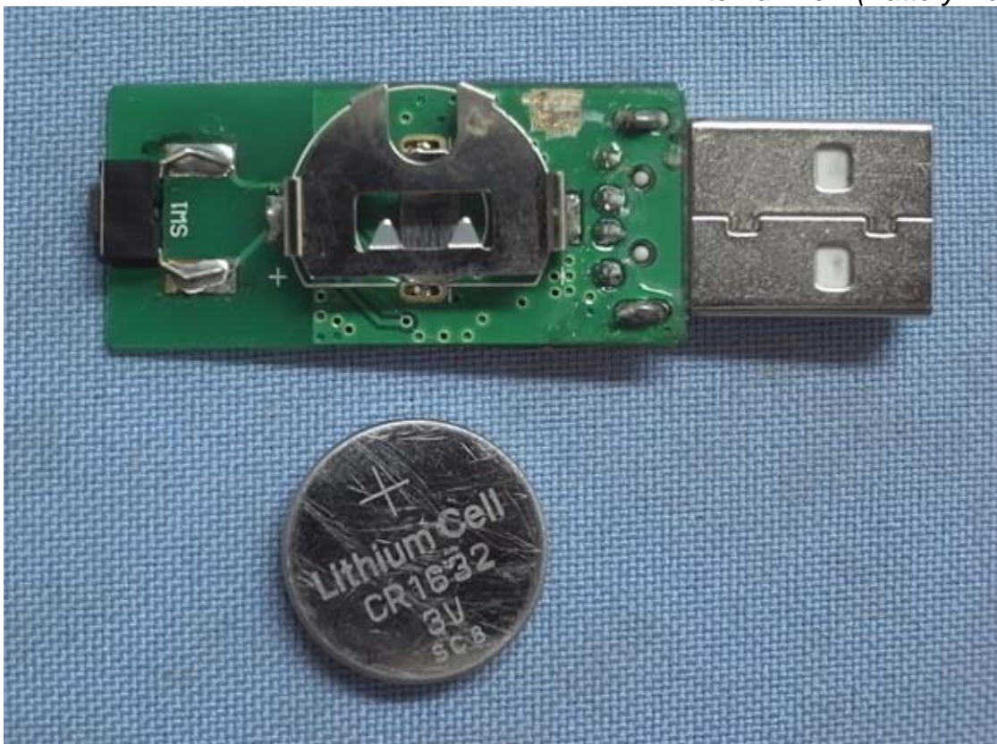
Photo 4 Internal View (Battery Removed)
