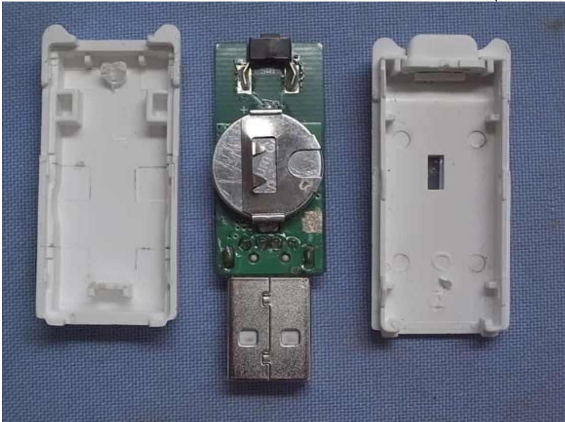
Photo 3 Internal View (Cover Removed)
