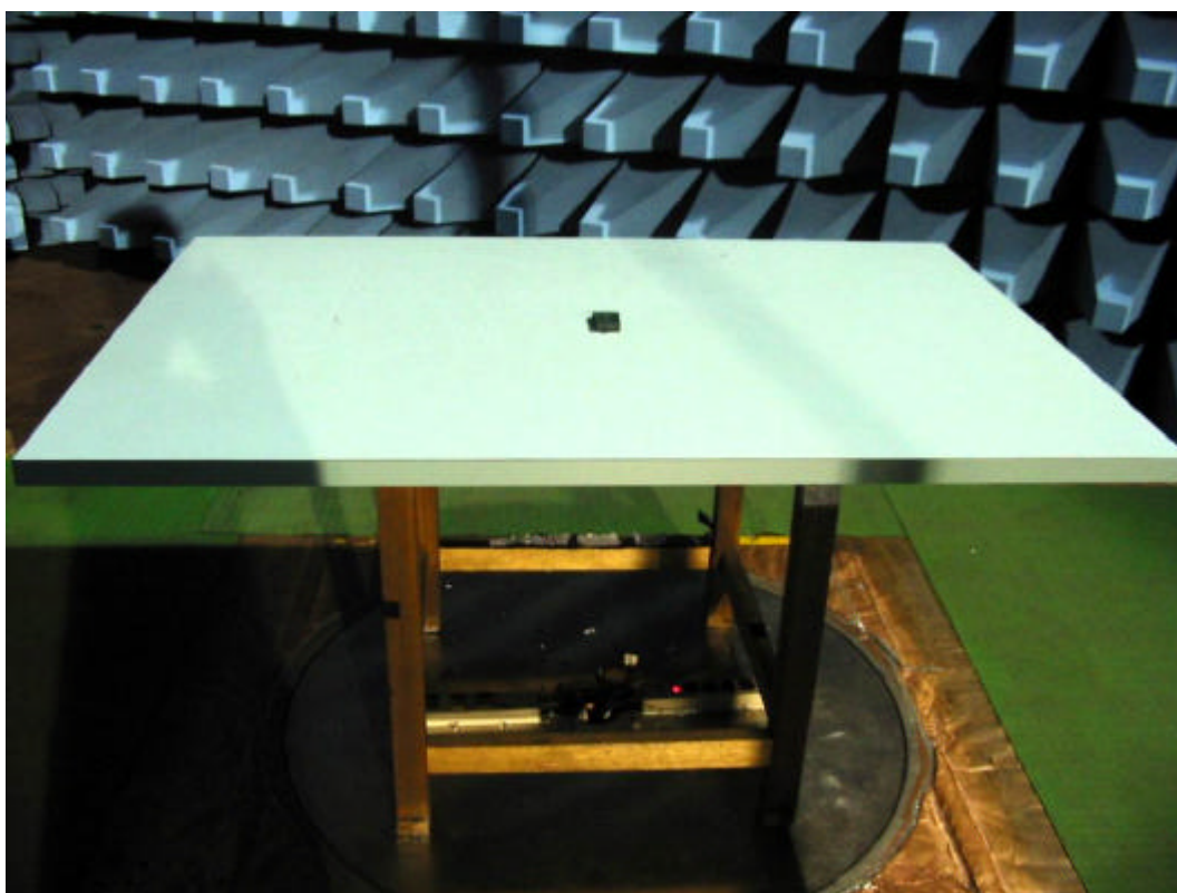
The Test configuration of Rear view of X-axis
