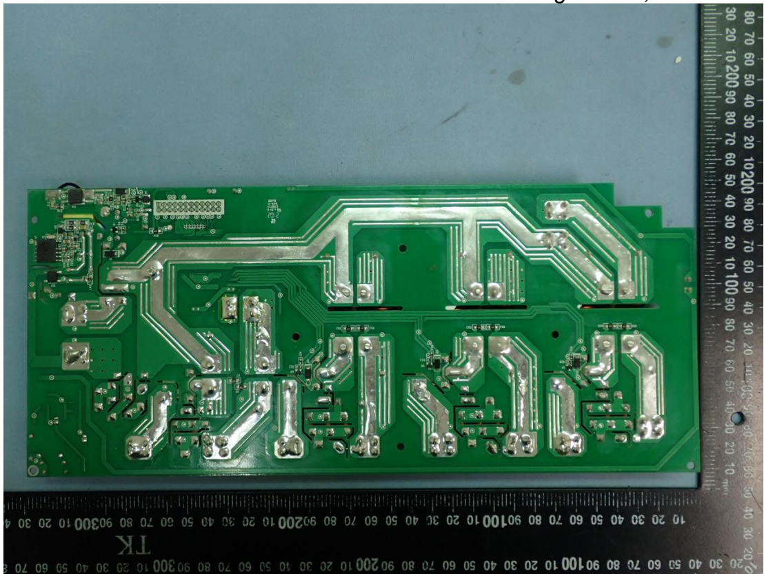
Figure 9 Surge Board, Back View
