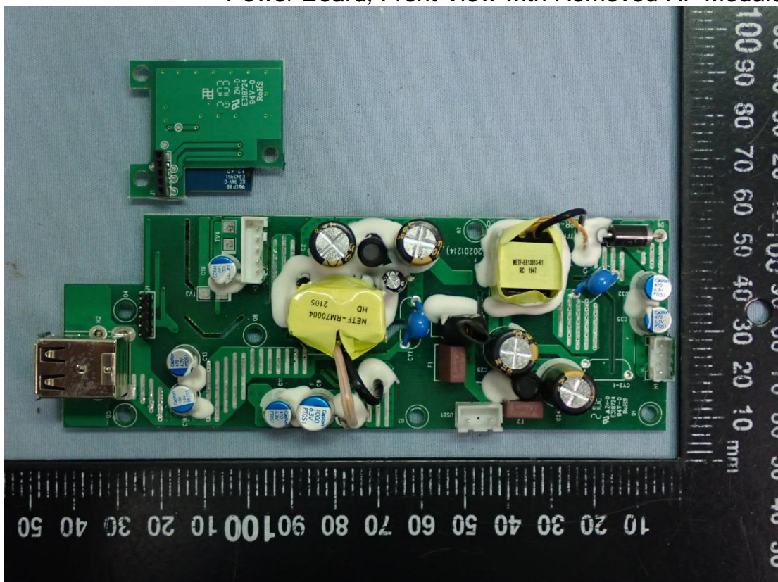
Figure 14 Power Board, Front View with Removed RF Module
