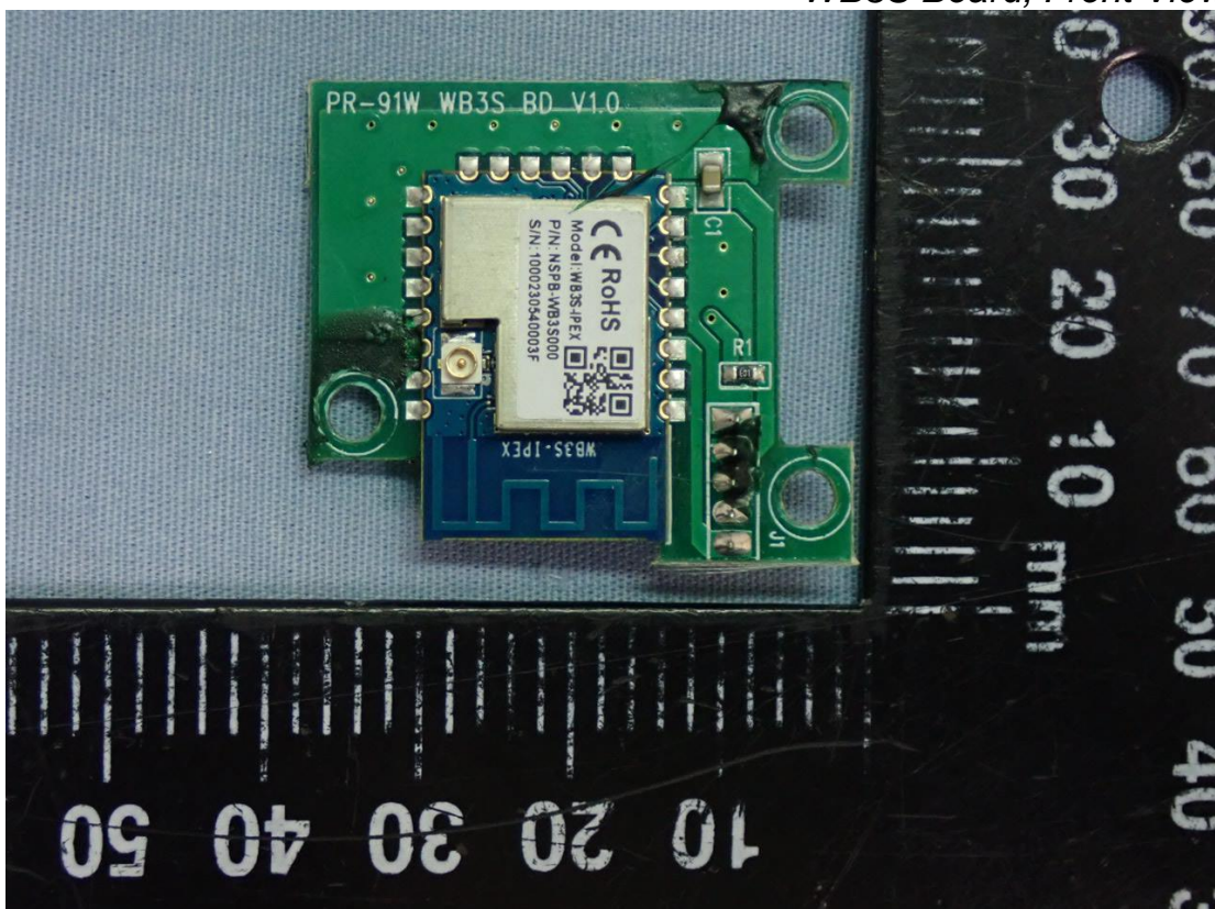
Figure 16 WB3S Board, Front View
