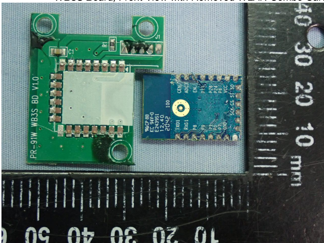
Figure 18 WB3S Board, Front View with Removed WLAN Combo Card
