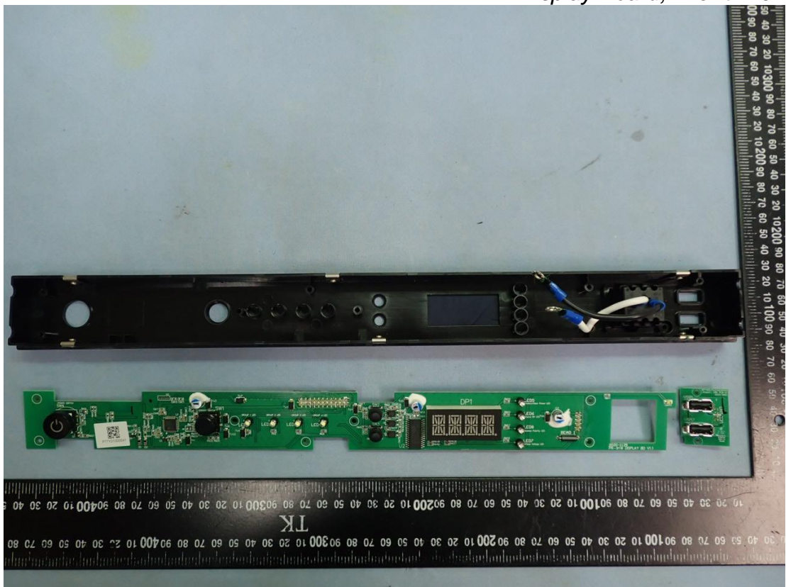
Figure 10 Display Board, Front View
