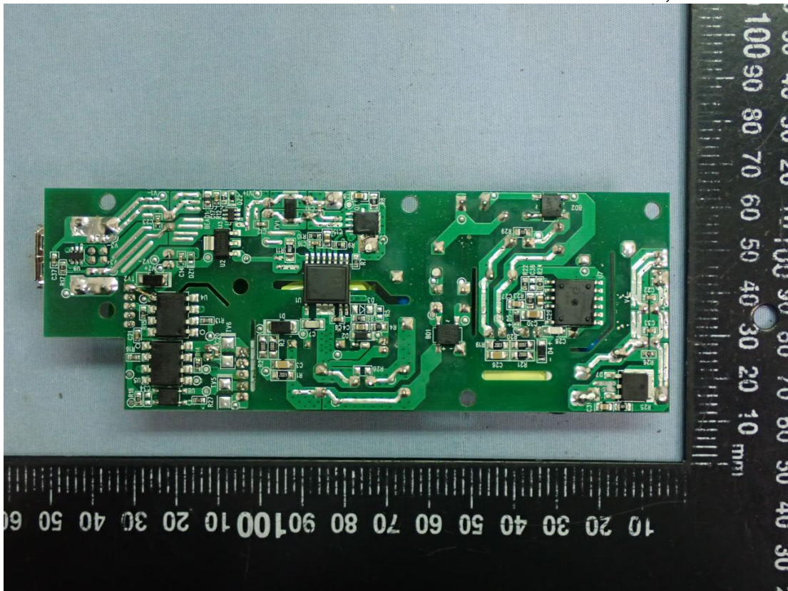
Figure 15 Power Board, Back View
