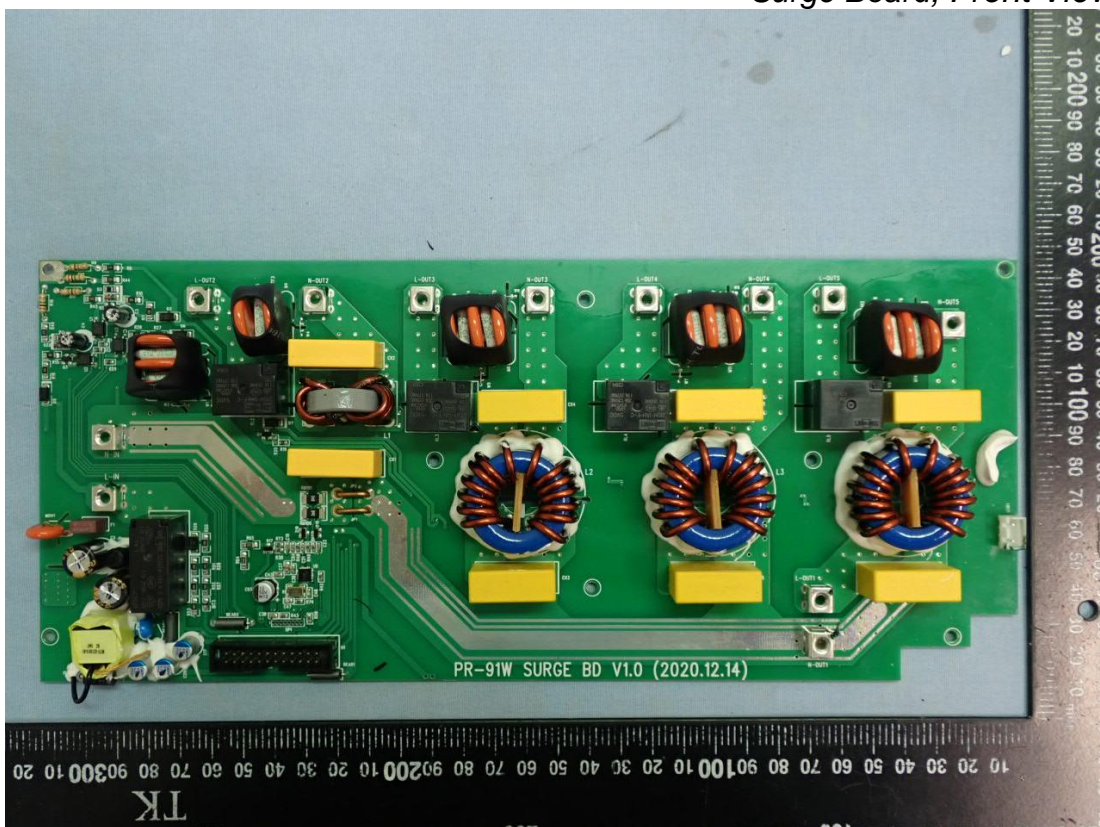
Figure 8 Surge Board, Front View
