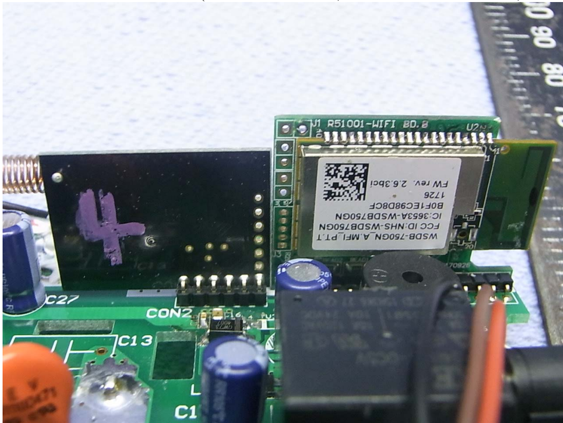
Figure 11 Internal View (WiFi-MCU Module, Front View and RF Board, Back View)
