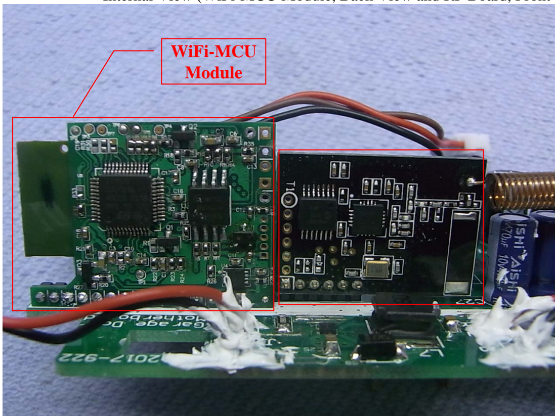
Figure 12 Internal View (WiFi-MCU Module, Back View and RF Board, Front View)
