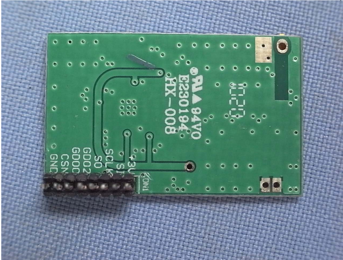
Figure 9 Internal View (Internal Board, Back View)
