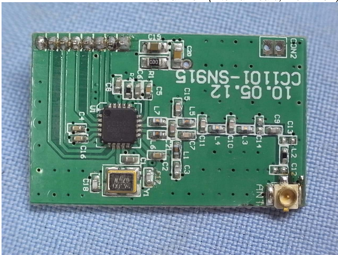
Figure 8 Internal View (Internal Board, Front View)
