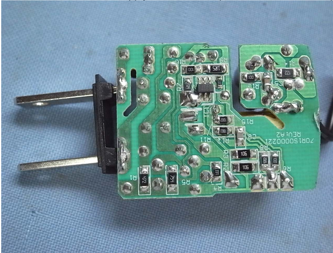
Figure 13 I.T.E Power Supply, Internal View (Main Board, Back View)
