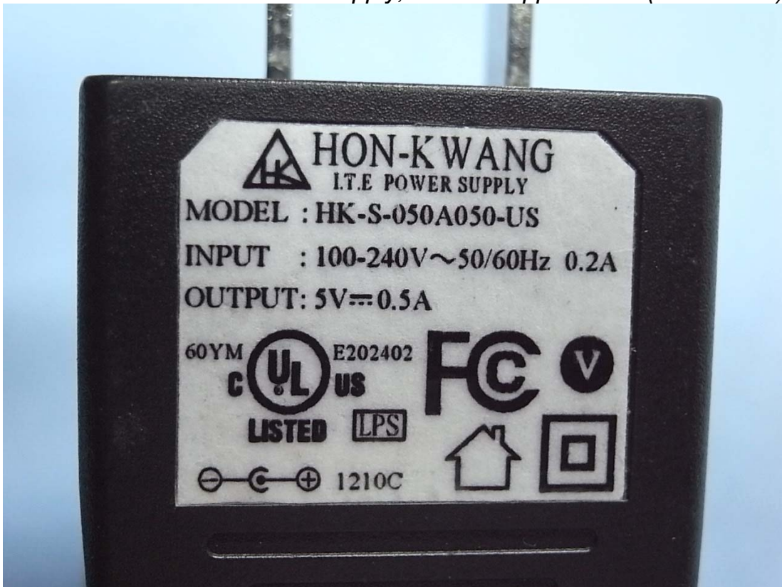
Figure 4 I.T.E Power Supply, General Appearance (Label View)
