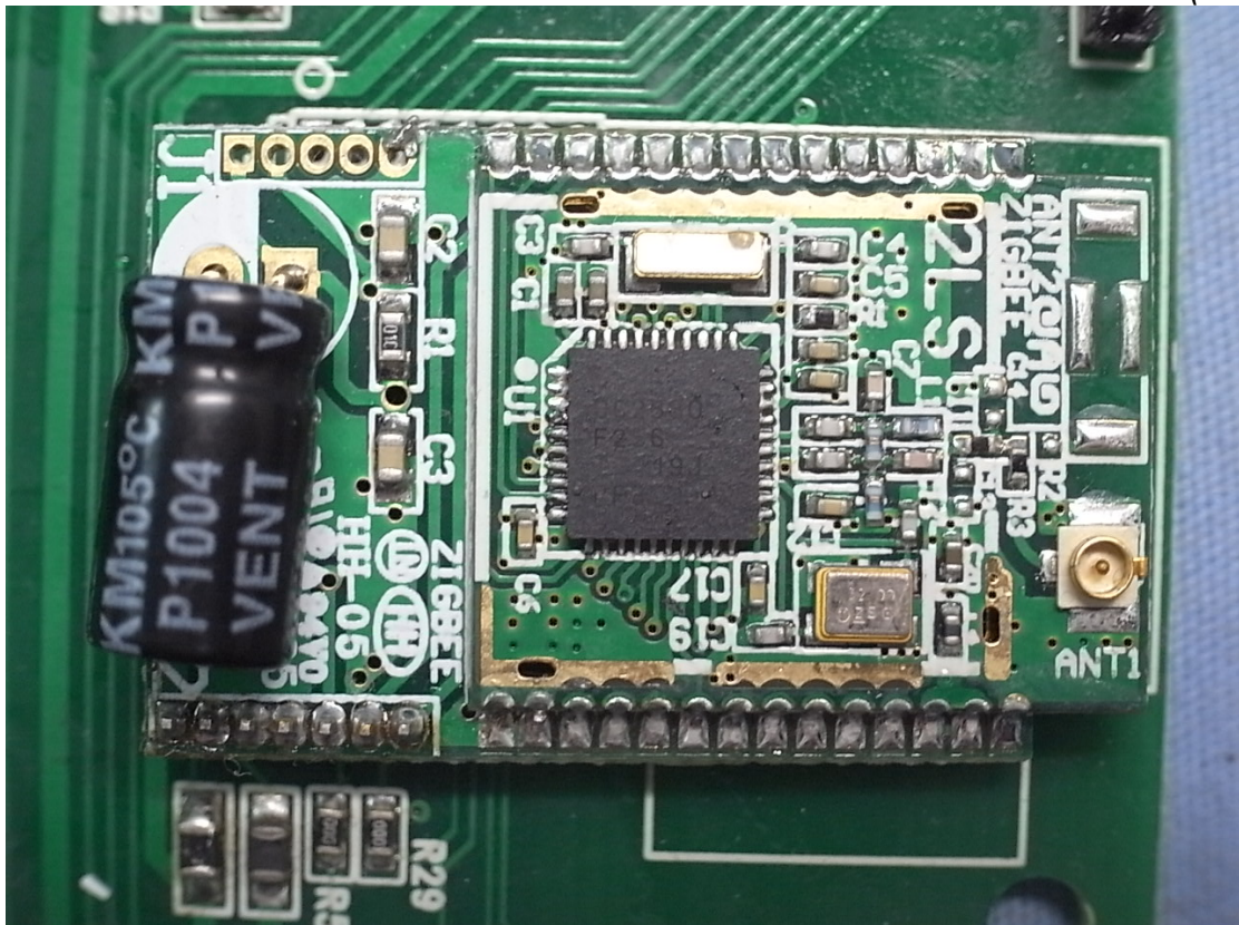
Photo 10 Internal View (RF Board)
