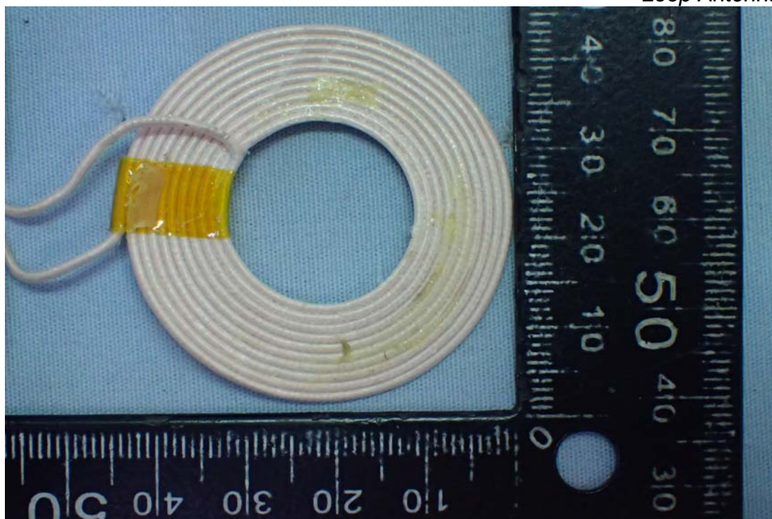
Figure 6 Loop Antenna
