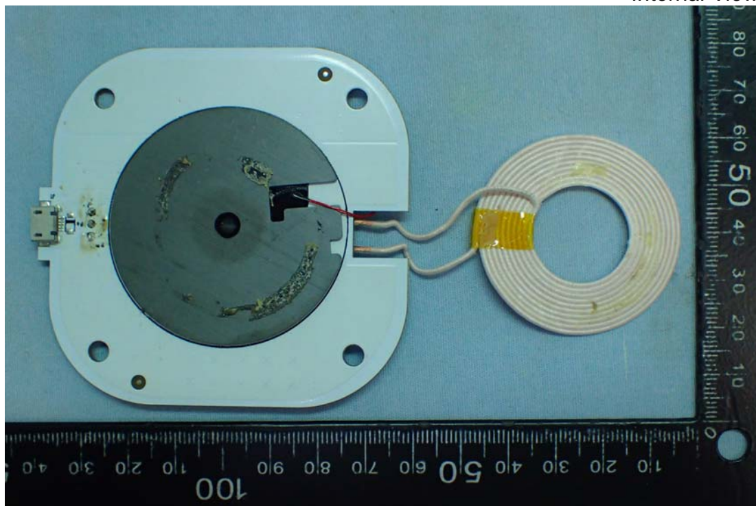
Figure 5 Internal View
