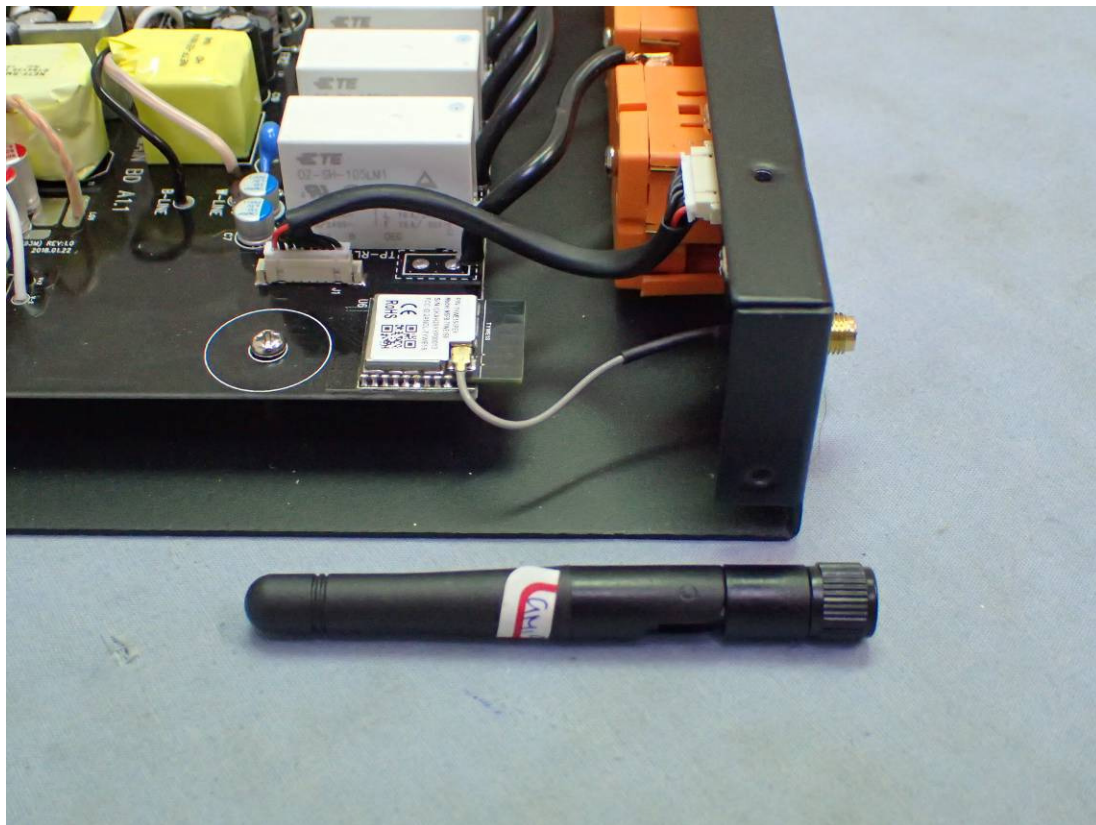
Figure 10 Internal View
