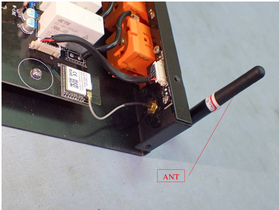
Figure 9 Internal View
