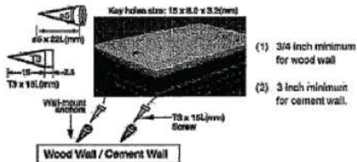
Figure 1. Mounting on a Wall
