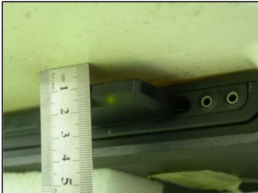
The bottom of the EUT face to the phantom with 10mm-separation distance.
