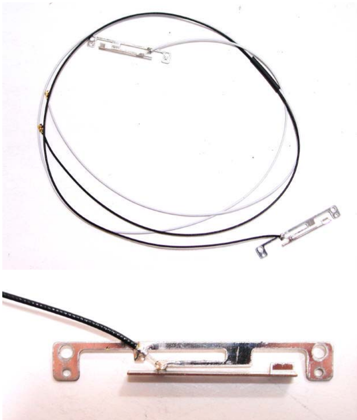
Antenna#4
