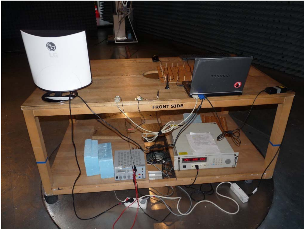
Photo 1: Test setup for radiated measurements (Computer setup Part 15b above 30 MHz)
