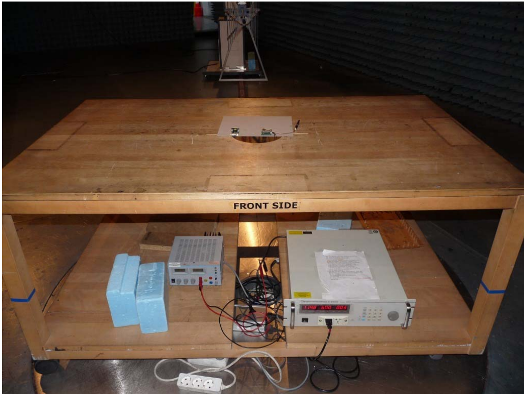
Photo 4: Test setup for radiated measurements Part 15.247 (Enclosure, below 1 GHz)
