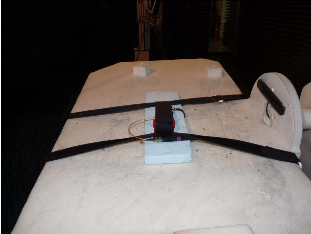
Photo 5: Test setup for radiated measurements Part 15.247 (Enclosure, above 1 GHz)
