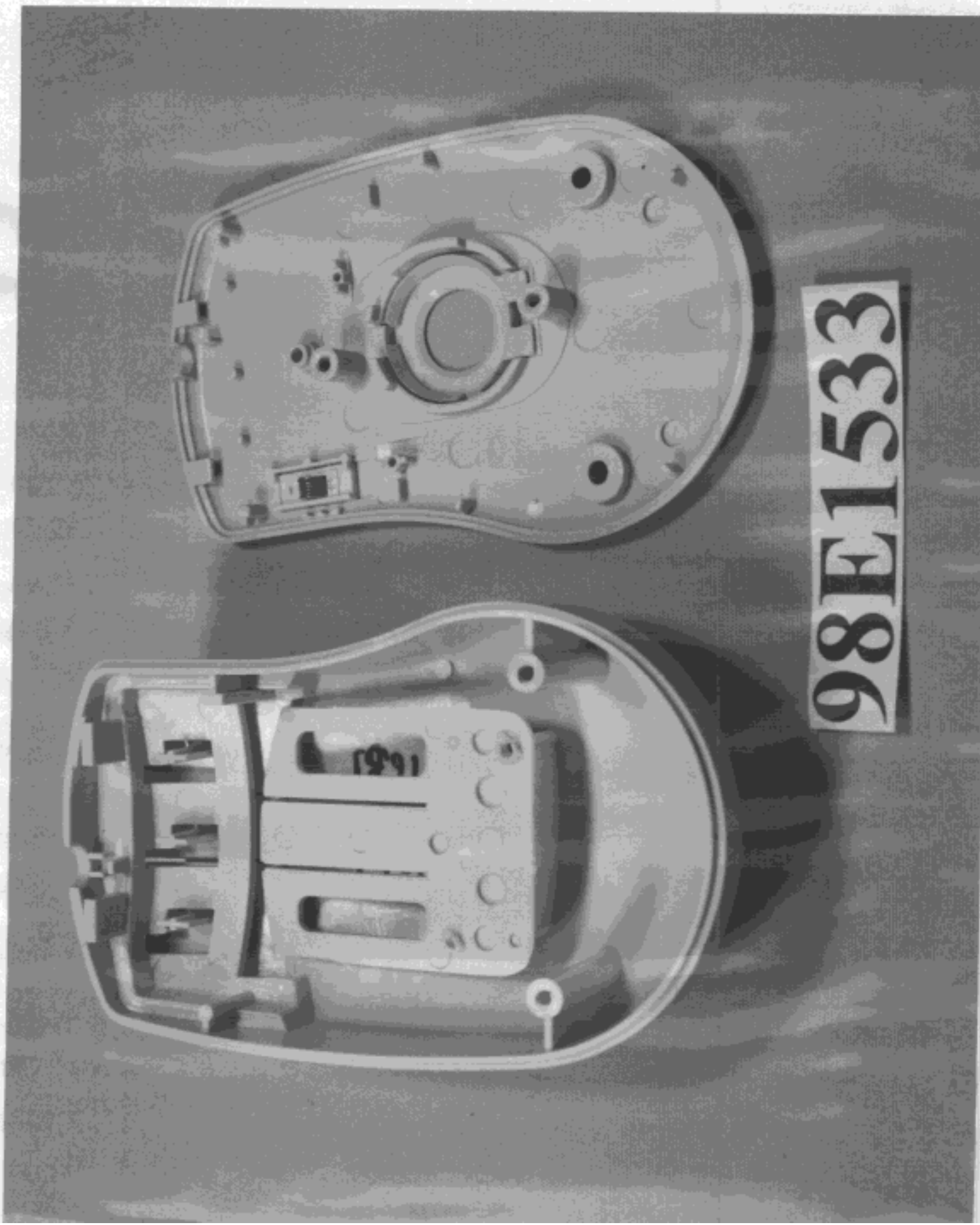
Photo # 12. SP3000 Unit Partially Disassembled
