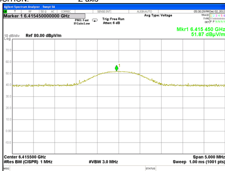
Plot 7.2.22 Radiated emission measurements at the seventh harmonic frequency
