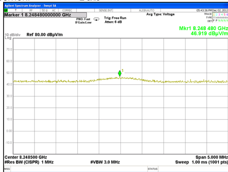
Plot 7.2.26 Radiated emission measurements at the ninth harmonic frequency
