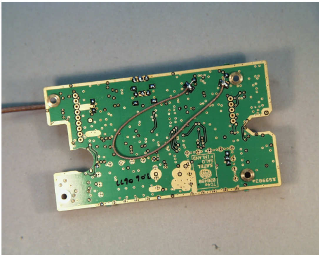
Fig. 8 : RF PCB, Bottom View (identical to Sateline 3AS)
