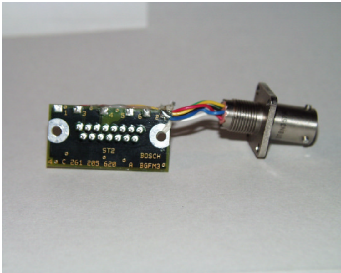
Fig. 10 : Adaptor Board, Bottom View
