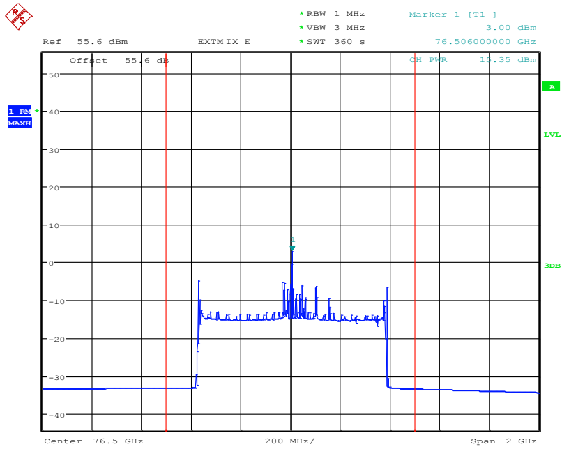
Plot 13: Sample 6 , EIRP (Average detector), T_{nom} / V_{nom} , normal mode
