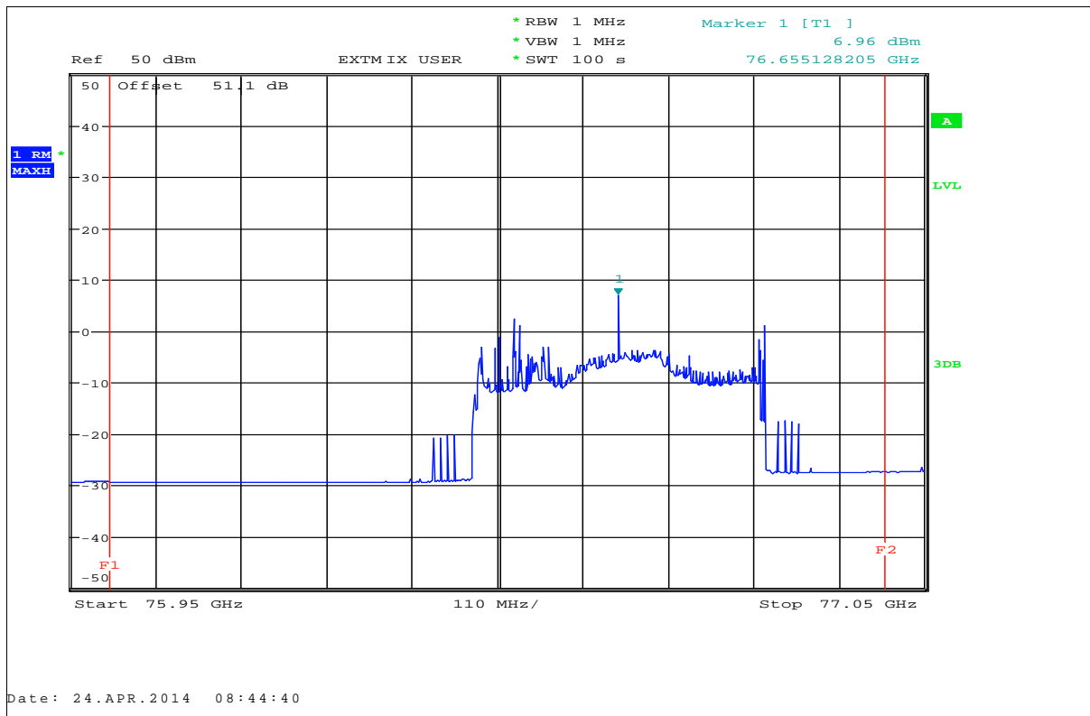
Plot 4: EIRP (RMS detector), T_{min} / V_{min} - V_{max} ,
