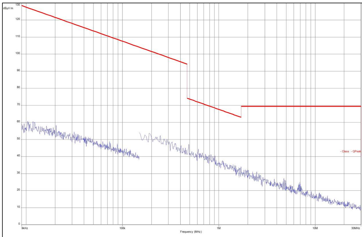
Plot 7: 9 kHz – 30 MHz, magnetic loop antenna, valid for all frequencies
