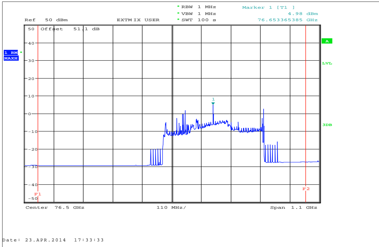
Plot 6: EIRP (RMS detector), T_{max} / V_{min} - V_{max} ,
