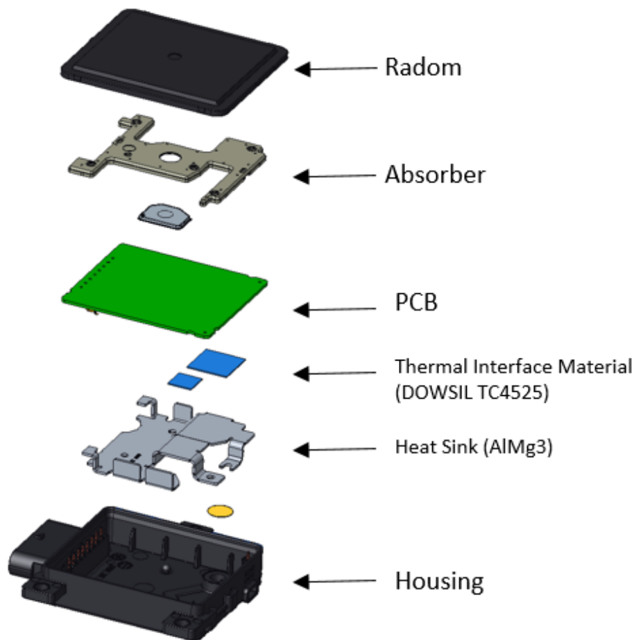
Figure 1: FR5TPCC assembly view
