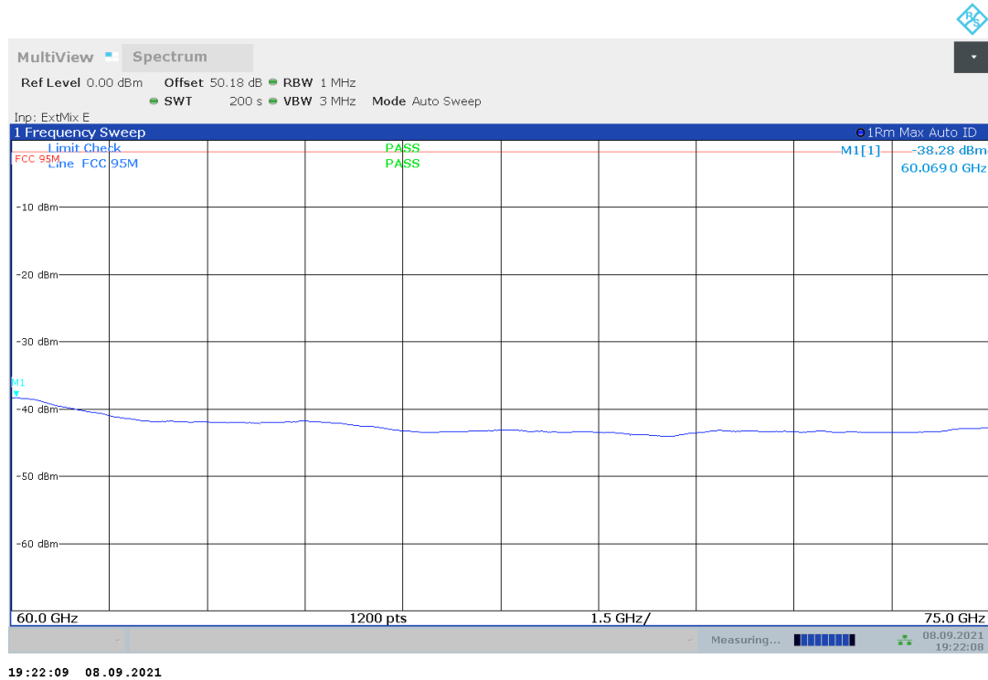
Plot no. 22: radiated emissions 60 GHz – 75 GHz, mode 7, polarization vertical / horizontal
