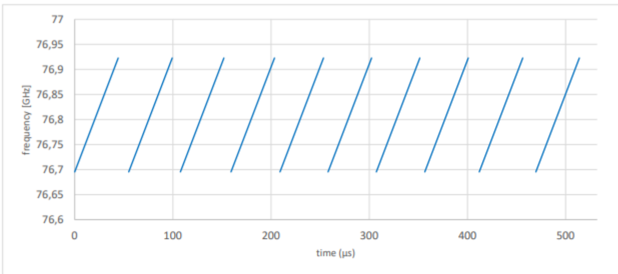
Figure 6: Dingle sequence
