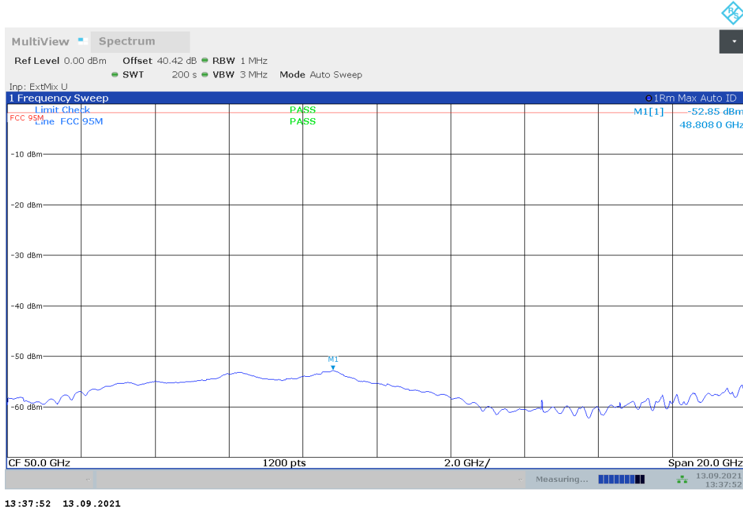
Plot no. 21: radiated emissions 40 GHz – 60 GHz, mode 7, polarization vertical / horizontal
