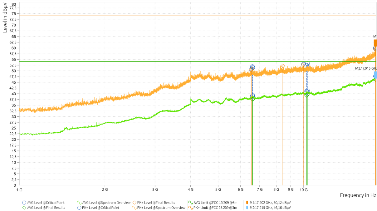
Plot no. 53: radiated emissions 1 GHz – 18 GHz, mode 8, polarization vertical / horizontal Spectrum Overview
