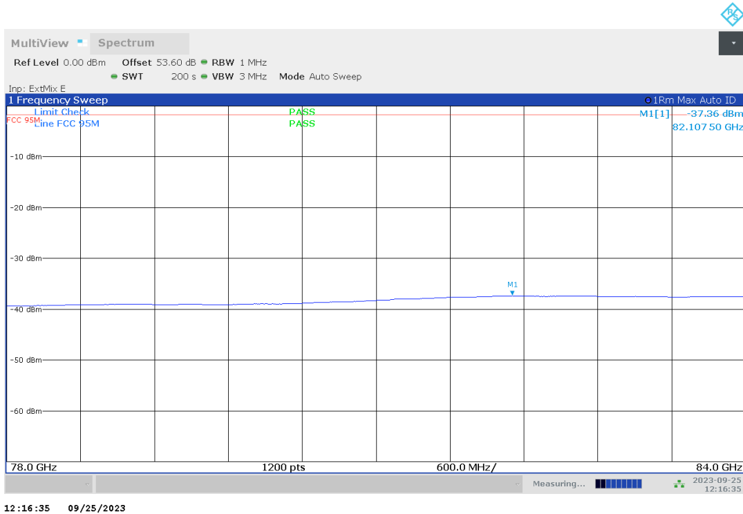
Plot no. 74: radiated emissions 78 GHz – 84 GHz, mode 8, polarization vertical / horizontal
