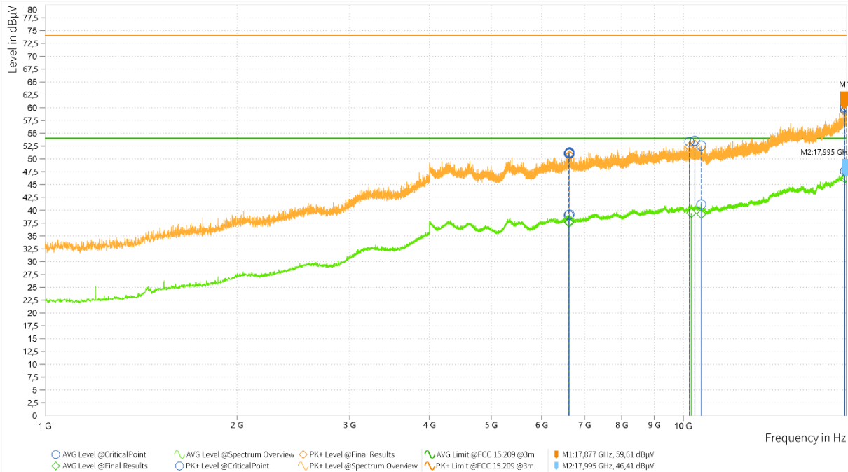
Plot no. 54: radiated emissions 1 GHz – 18 GHz, mode 9, polarization vertical / horizontal Spectrum Overview
