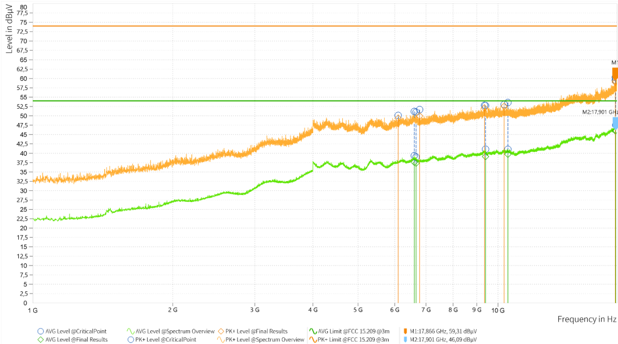
Plot no. 52: radiated emissions 1 GHz – 18 GHz, mode 7, polarization vertical / horizontal Spectrum Overview
