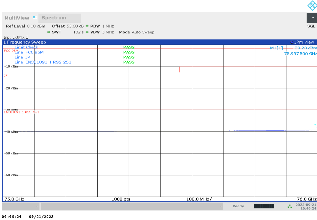
Plot no. 69: radiated emissions, Band edge Low, mode 9, polarization vertical / horizontal
