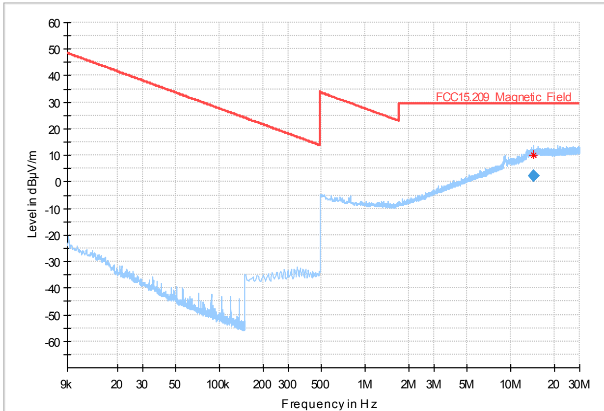
Plot no. 46: radiated emissions 9 kHz – 30 MHz, mode 7, loop antenna
