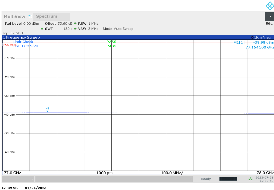
Plot no. 72: radiated emissions, Band edge High, mode 9, polarization vertical / horizontal
