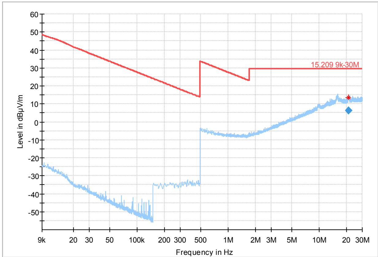
Plot no. 47: radiated emissions 9 kHz – 30 MHz, mode 8, loop antenna
