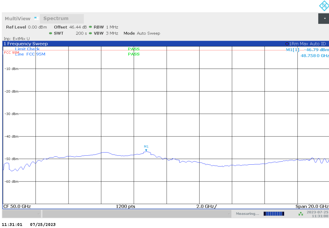
Plot no. 63: radiated emissions 40 GHz – 60 GHz, mode 9, polarization vertical / horizontal
