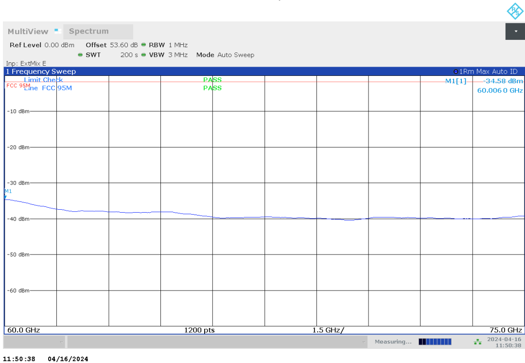
Plot no. 53: radiated emissions mode 2, 60 GHz – 75 GHz, polarization vertical / horizontal
