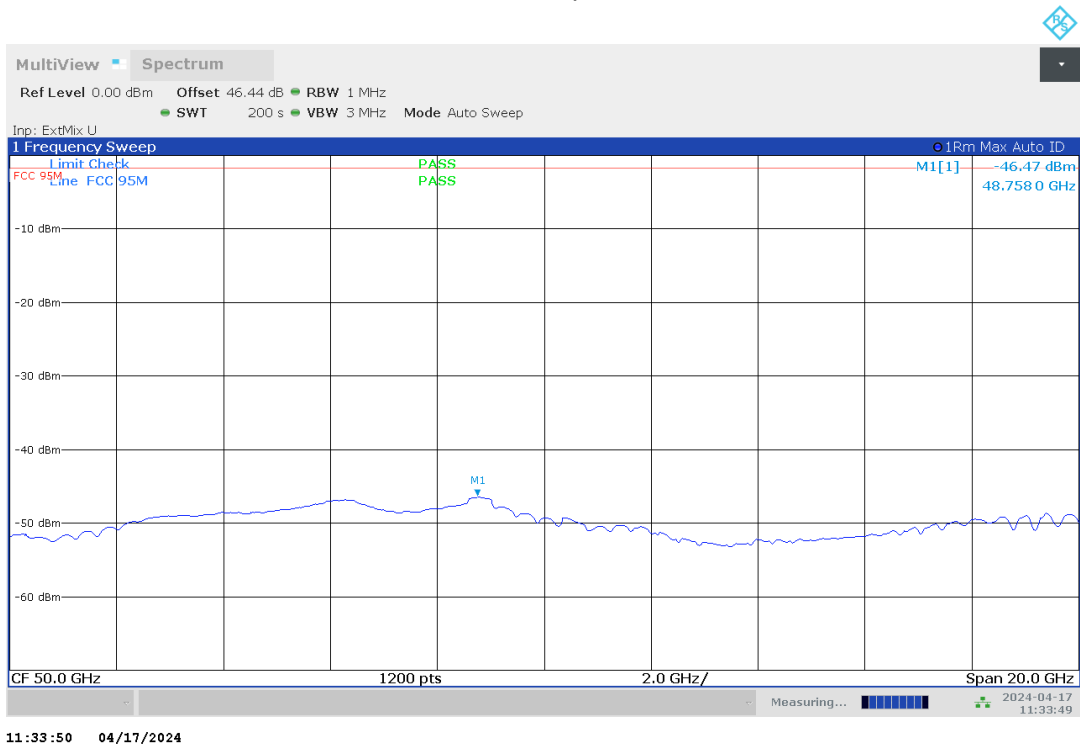
Plot no. 52: radiated emissions mode 2, 40 GHz – 60 GHz, polarization vertical / horizontal
