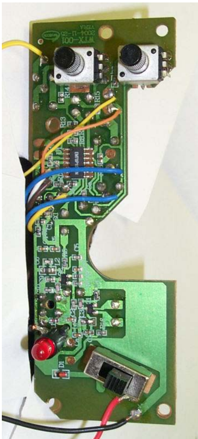
Component Side
