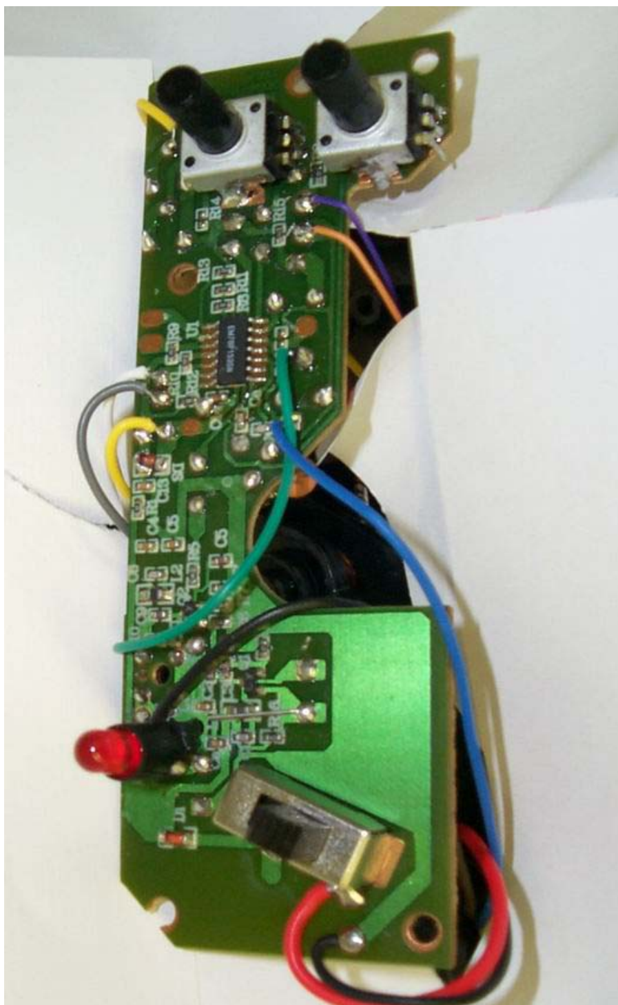
Component Side
