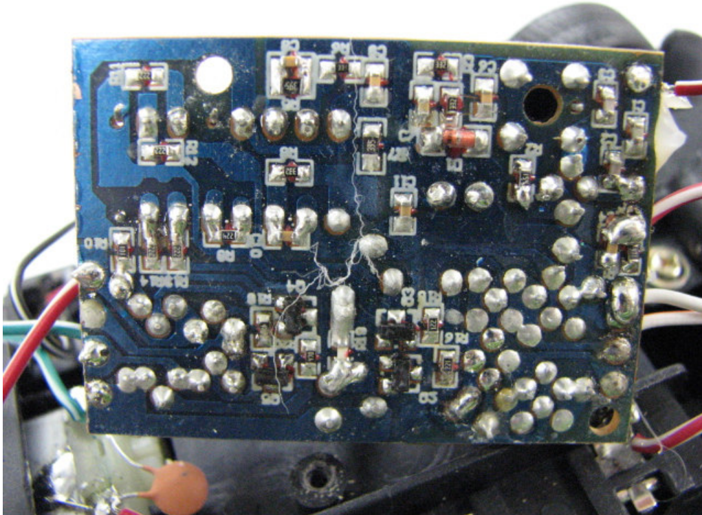
Receiver (Internal view)
