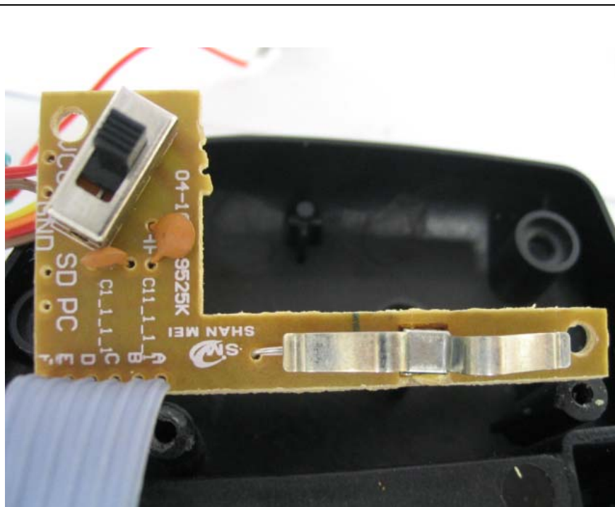
Transmitter (Internal view)
