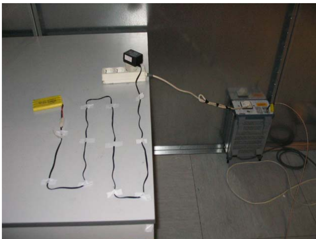
Set-up for Conducted Emission test
