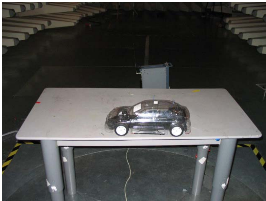
Set-up for Radiation Emission ( Receiver)
