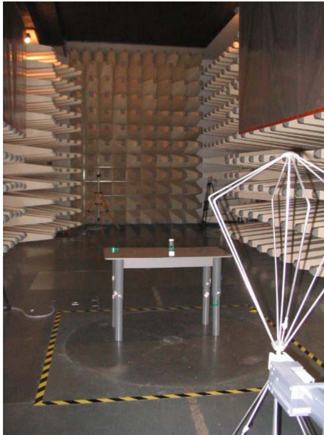
Set-up for Radiation Emission ( Transmitter)
