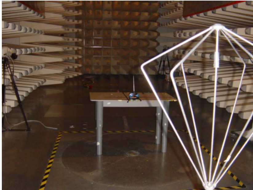
Set-up for Radiation Emission (Transmitter)
