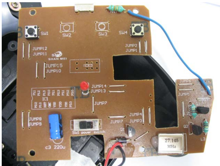
Transmitter (Internal view)
